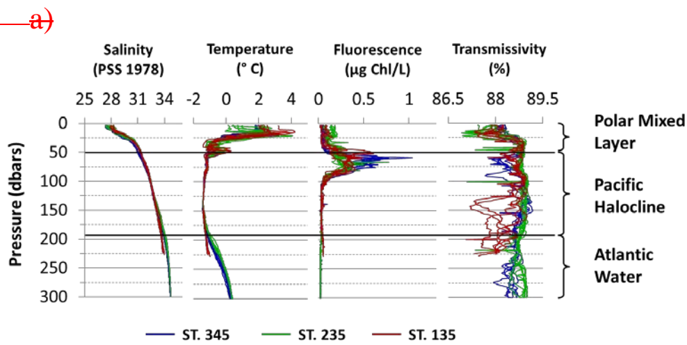
Figure 3. Environmental and mooring parameters: a) Vertical profiles of salinity, temperature, fluorescence and transmissivity and main water masses at the three sites of drifting trap deployment; b) Mooring configuration including sediment trap depths and horizon of maximum chlorophyll-a.
