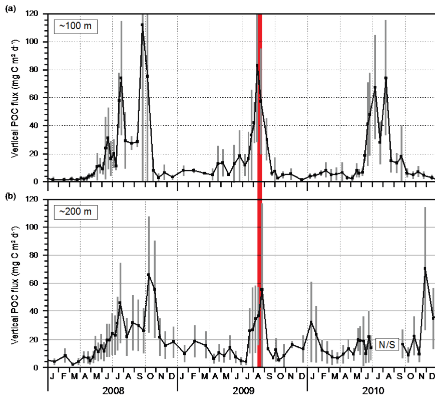
Figure 56. Times series of mean downward POC fluxes as measured at (a) ~100 m and (b) ~200 m with the ArcticNet sequential sediment traps (A1, G09, CA05, CA08 and CA16) moored in the vicinity of the drifting stations (see Fig. 1, Table 2). Vertical grey bars depict the standard deviation associated with each mean POC flux data point. The vertical red bar delimits the third week of August 2009 when short-term traps were deployed. N/S: no sampling.
