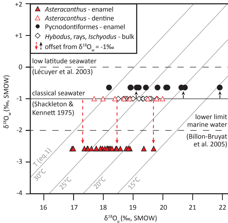
Figure 4. \delta^{18}\text{O}_p values of Porrentruy fish samples and related water temperature ( T ) resulting from Eq. (1). Hybodius , rays, Ischyodus as well as most Asteracanthus dentine samples are considered diagenetically altered. Arrows show effect of varying \delta^{18}\text{O}_w in Eq. (1) from classical seawater value ( -1\text{‰} ). Realistic and consistent temperatures for Asteracanthus and Pycnodontiformes imply the influence of respectively distinct paleoenvironments.
