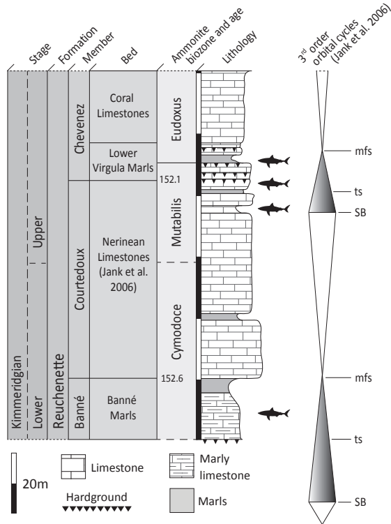
Figure 2. Simplified stratigraphic profile of the Porrentruy area with third order orbital cycle and section yielding the studied chondrichthyan material. Numbers indicate geological age in millions of years. SB = sequence boundary, ts = transgressive surface, mfs = maximum flooding surface.
