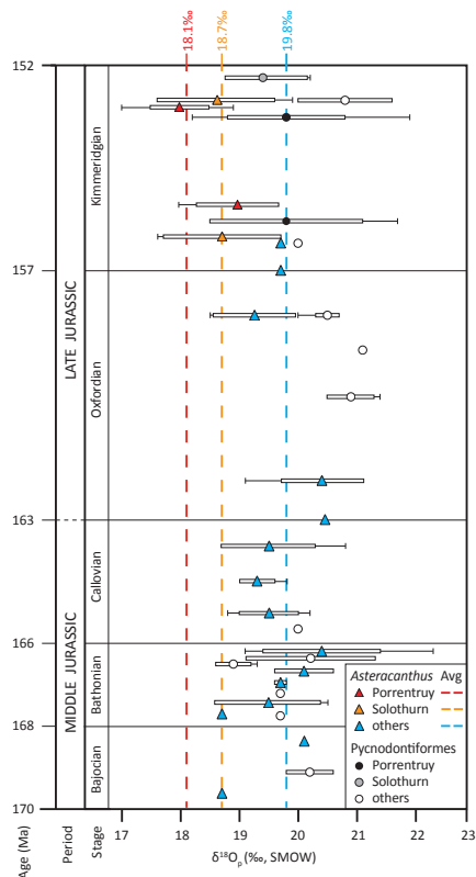
Figure 5. Comparison of \delta^{18}\text{O}_p values (average, standard deviation, end members) of Pycnodontiformes and Asteracanthus enamel samples from Porrentruy, Solothurn and other European localities through time. The approximate geographical position of previously studied localities (Dromart et al., 2003; Lécuyer et al., 2003; Billon-Bruyat et al., 2005) is shown in Fig. 1. Detailed localities are available in the Supplement.
