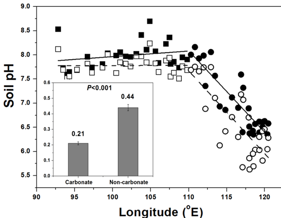
Figure 2. Effects of acid addition ( 16 \text{ mmolH}^+ \text{ kg}^{-1} soil) (approximately the average cumulative amount of acid deposited over 10 years) on soil pH in the carbonate containing soils (squares) and the non-carbonate containing soils (circles). Mean changes in pH (i.e. decrease) of carbonate and non-carbonate soils are shown in inset. Black symbols (and solid line) and white symbols (and dashed line) represent control and acid-treated soils, respectively.
