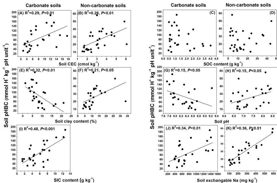
Figure 3. Relationships between soil pH buffering capacity (pHBC) and soil variables (cation exchange capacity (CEC), soil organic carbon (SOC), soil clay content, soil pH, soil inorganic carbon (SIC), and soil exchangeable sodium (Na)) in the carbonate containing soils and non-carbonate containing soils. All the regression results are referred to Table 2.
