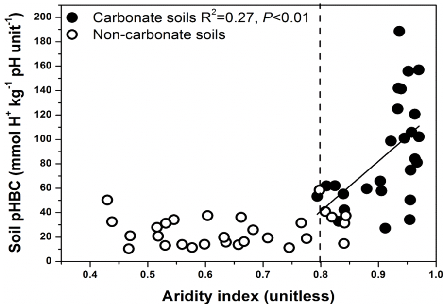
Figure 4. Relationships between soil pH buffering capacity (pHBC) and aridity index in the carbonate containing soils (solid circles) and the non-carbonate containing soils (empty circles). Dashed line represents the boundary between the arid regions (aridity index > 0.8) and the semi-arid regions (aridity index < 0.8). All the regression results are referred to Table 2.
