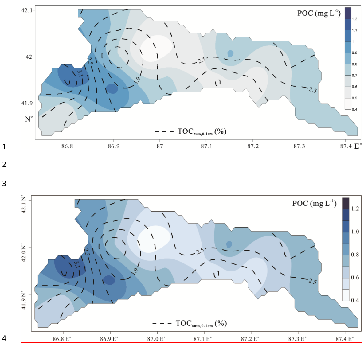
5 Figure 7. Spatial distributions of (a) POC concentrations in summer (color map) and 6 (b) autochthonous TOC in the 0-1 cm sediment ( \text{TOC}_{\text{auto } 0-1\text{cm}} , dashed lines). POC data 7 were from Wang et al. (2014).
