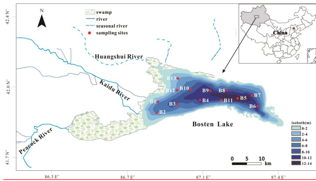
4 Figure 1. Map of the Bosten Lake with the water depth and the 13 sampling stations 5 (red dots). Bathymetric was measured in 2008 by Wu et al. (2013) and bathymetric 6 contours were plotted by using software ArcGIS 9.3 and Corel DRAW X3.
