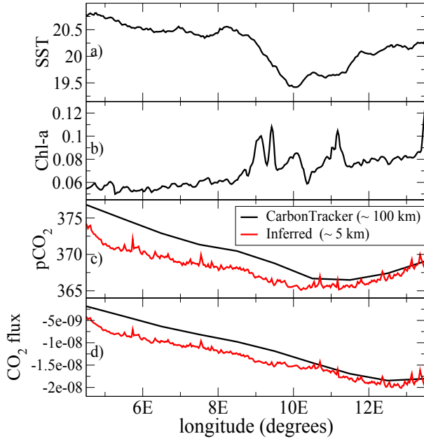
Fig. 6. Longitudinal profiles of a) SST from OSTIA products in units of °C, b) Chl from GLOBCOLOUR-GSM ocean in mg/m 3 , c) pCO_2^{CTrack} (black line) and pCO_2^{infer} (red line) in \mu\text{atm} , and d) air-sea CO 2 fluxes from CarbonTracker (black line) and inferred air-sea CO 2 fluxes (red line) in mol C m -2 s -1 . All these longitudinal profiles correspond to the fixed latitude equal to 33.5°S of the plots shown in Fig. 5 for March 22, 2006.
