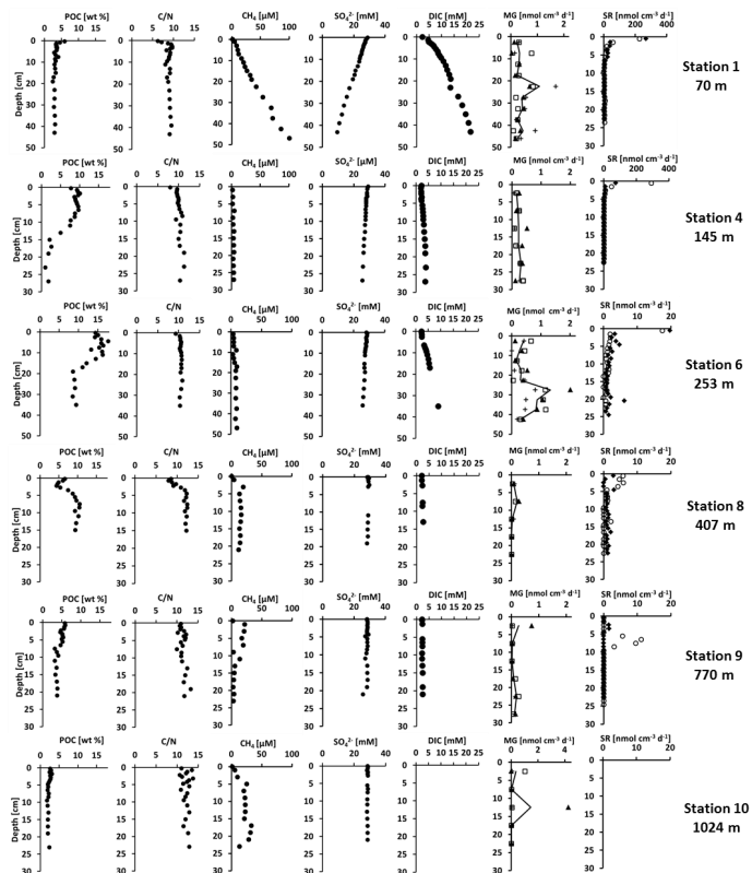
Figure 2. Profiles of particulate organic carbon (POC), C/N ratio, methane (CH 4 ), sulfate (SO 4 2- ), DIC (dissolved inorganic carbon), net methanogenesis (MG) rates and sulfate reduction (SR) rates in the MUC cores along the depth transect. For MG, triplicates (symbols) and mean (solid line) are shown. For SR, duplicates are shown. Data points from the overlying water in the MUC core (OLW) are set to 0 cm. Note deviant scale dimension for MG at St. 10 and for SR at St. 1 and 4.
