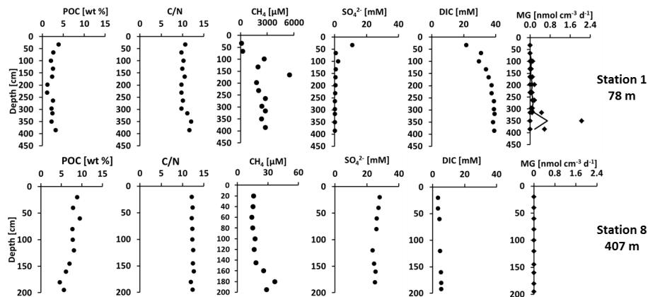
Figure 5. Profiles of particulate organic carbon (POC), C/N ratio, methane ( \text{CH}_4 ), sulfate ( \text{SO}_4^{2-} ), dissolved inorganic carbon (DIC), and hydrogenotrophic methanogenesis (MG) rates in the gravity cores at two stations within the depth transect. For MG, triplicates (symbols) and mean (solid line) are shown.
