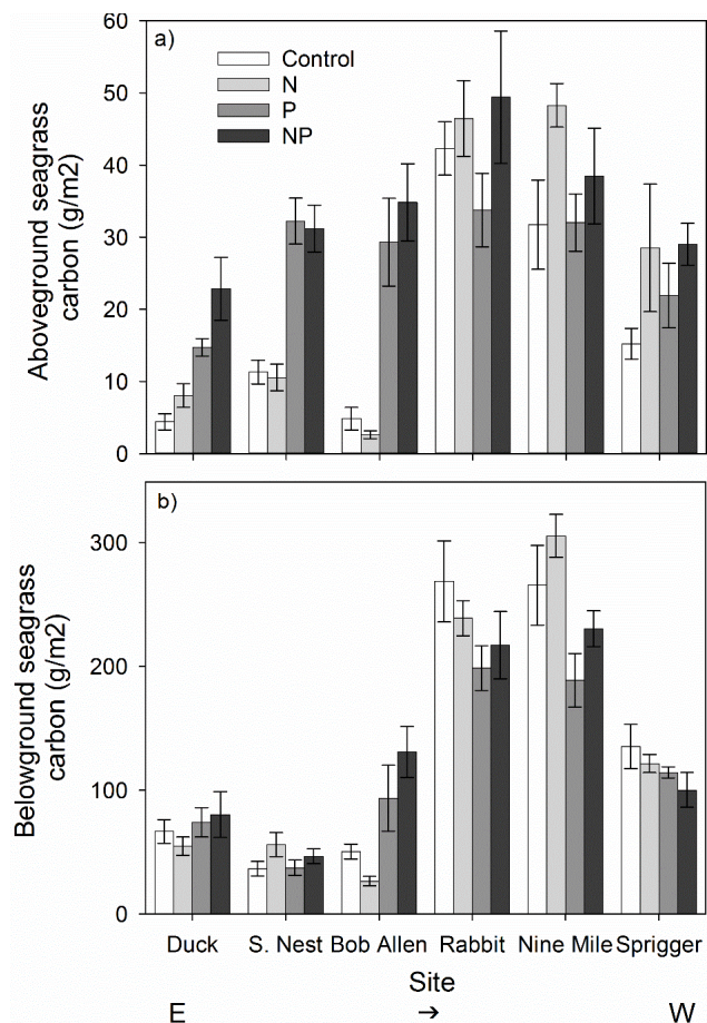
Figure 2. (a) Aboveground and (b) belowground seagrass carbon stocks at six sites in response to nitrogen (N) and phosphorus (P) addition. Sites are displayed along a naturally occurring P-availability gradient from low P availability in the east to high P availability in the west.
