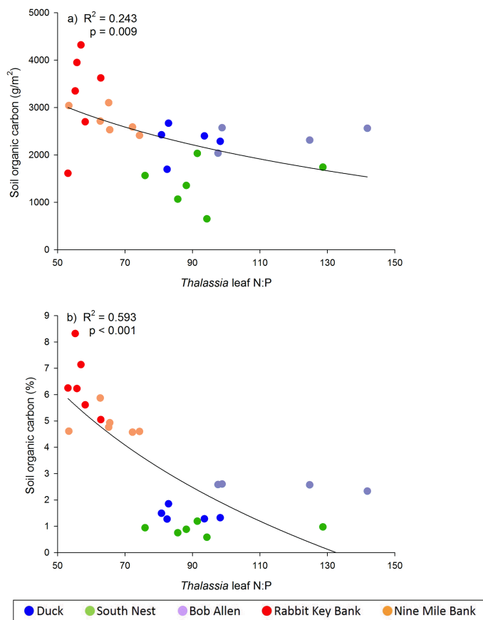
Figure 4. Logarithmic relationship between Thalassia testudinum leaf N : P ratio and soil carbon stock in control plots, reported in (a) \text{g m}^{-2} and (b) percent. Sites are listed in the legend in order from east (most P limited) to west (least P limited).
