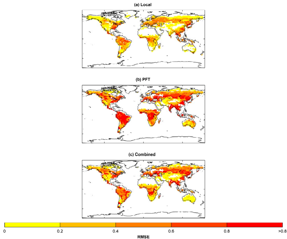
Figure 1. Root mean squared error (RMSE) of predicted LAI over the model study period for the local, PFT and combined models. All values have been normalised to the mean observed LAI at all locations.
