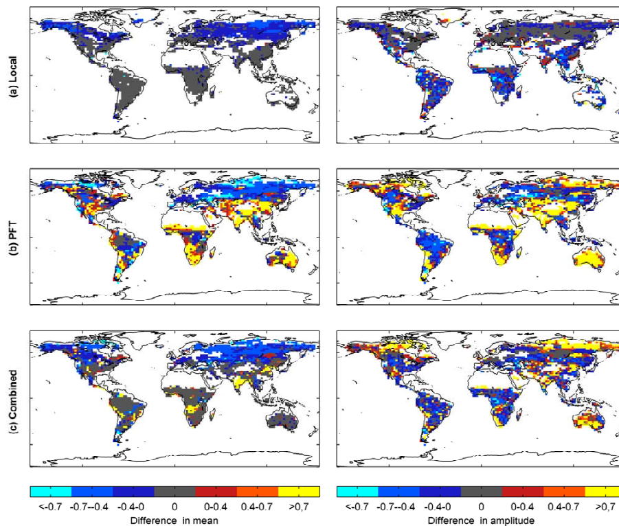
Figure 2. Difference between predicted and observed annual mean LAI (left) and seasonal amplitude (right) for the local, PFT and combined models. All values have been normalised to the mean observed LAI at all locations.
