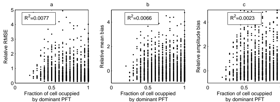
Figure 6. Correlations between model error and fraction of each grid occupied by the dominant PFT as a proxy for grid heterogeneity. (a) Model RMSE, (b) bias in LAI mean and (c) bias in LAI amplitude.
