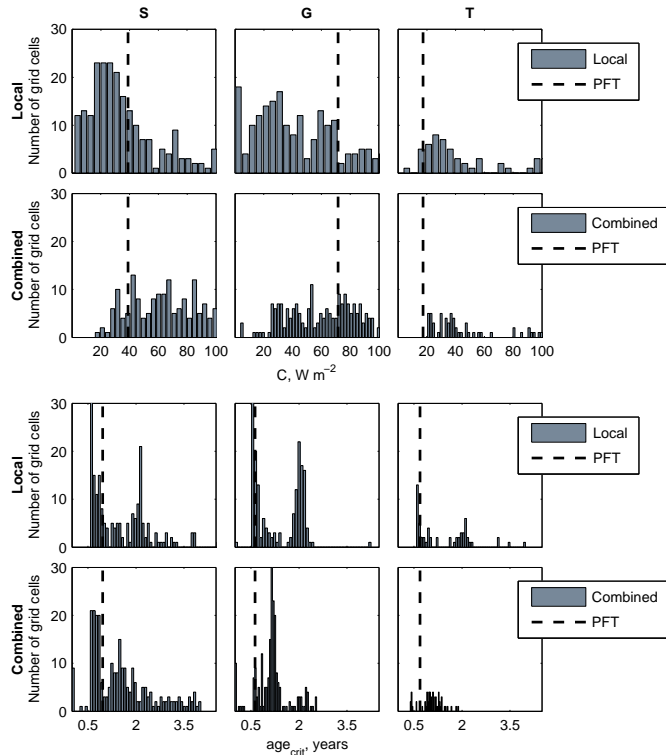
Figure 8. Parameter distributions for the light compensation point and age limit in three representative grass PFTs, savanna (S), grassland (G) and tundra (T). Parameter values are the mean of the fitted posterior distributions and the represented values reflect the variation in space within one PFT, for the local (top) and combined (bottom) models, as well as for the fitted PFT (black line).
