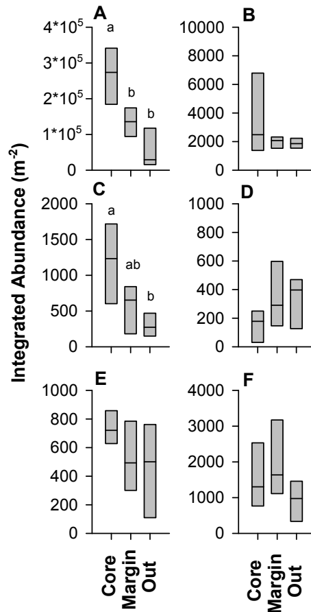
Figure 5. UVP5-derived integrated abundance (m -2 , upper 600 m) of large aggregates (>500 μm, a ), copepods ( b ), gelatinous plankton ( c ), shrimp-like micronekton (euphausiids/decapods, d ), phaeodaria ( e ) and collodaria ( f ) in the eddy core ( n = 4 profiles), eddy margin ( n = 4 ) and outside of the eddy ( n = 7 ). Different letters denote significant differences.
