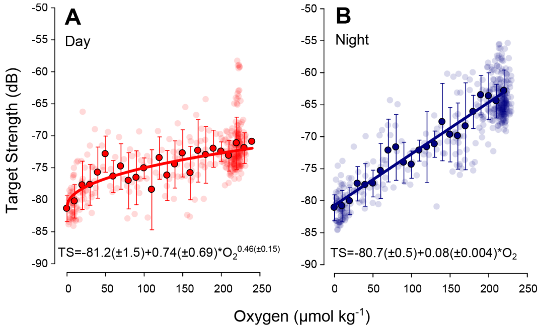
Figure 3. Moored ADCP (300 kHz, matched to depth of moored oxygen sensor) target strength (dB) as a function of oxygen concentration ( \mu\text{mol O}_2 \text{ kg}^{-1} ) during daytime ( a ) and nighttime hours ( b ). Higher target strength indicate a higher biomass of zooplankton and nekton. Transparent symbols are 1.5 hourly data, filled symbols are mean values ( \pm SD) for 10 \mu\text{mol O}_2 \text{ kg}^{-1} bins. Data are from 1 January to 14 March 2010.
