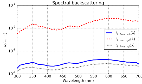
Figure 19. Spectral backscattering of the three test cases: homogeneous sphere, coated sphere and homogeneous cylinder.
