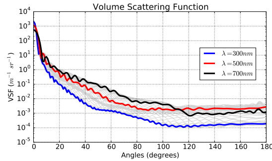
Figure 17. Volume scattering function obtained using the Bernard Model combined with Genetic Algorithm in the cylindrical example.
