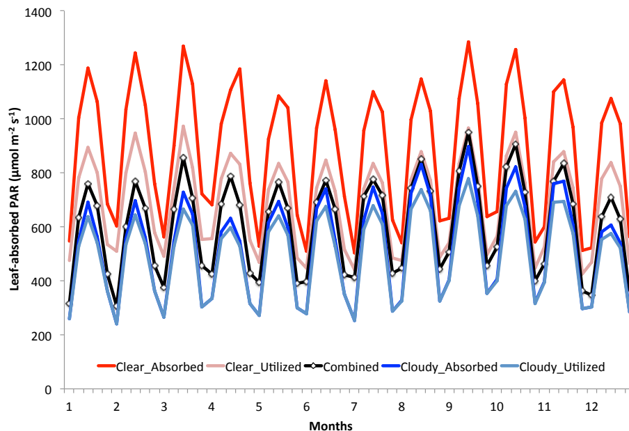
Figure 3. Cloudy (blue) and clear-sky DART simulations (red) were corrected for light saturation effects. Combined results (black line) are a weighted average of light utilization estimates from clear and cloudy simulations for five hours per day and one day per month.
