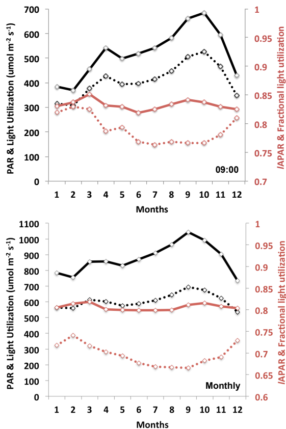
Figure 4. PAR (solid black) and modeled light utilization (dashed black) for DART simulations at 09:00LT (a, top) and monthly average values (b, bottom), based on a weighted average of hourly DART simulations. Simulated monthly values of /APAR (solid red) and fractional light utilization (dashed red) are plotted on the right-hand axis.
