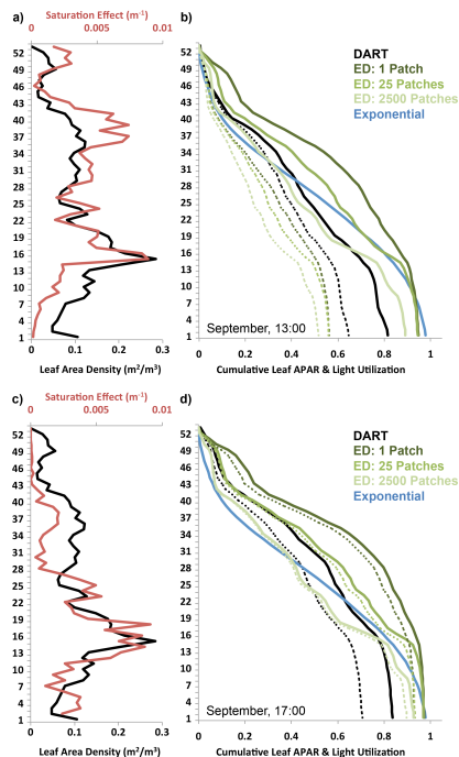
Figure 5. (a) Vertical profiles of leaf area density (black) and light saturation effect (red, difference between absorbed and utilized light) for September 13:00 LT DART simulations. (b) DART cumulative /APAR (black) and light utilization (dashed black) were compared to an exponential model of light extinction (blue, following Stark et al., 2012) and ED2 model simulations (green). Solid and dashed green lines depict cumulative leaf absorption and cumulative light utilization, respectively, for ED2 simulations with 1, 25, and 2500 patches. (c, d) Same as “(a)” and “(b)” for September 17:00 LT illumination conditions.
