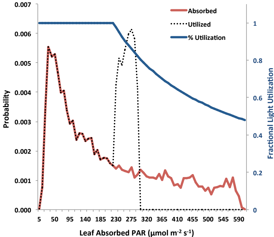
Figure 2. Probability distribution of leaf absorbed PAR (/APAR, red) and absolute light utilization (dashed black) for September 13:00 LT DART simulations. Light saturation effects reduce the effective leaf absorption > 225 \mu\text{mol m}^{-2} \text{s}^{-1} . Fractional light utilization (blue) for different /APAR values is plotted on the right y axis, based on leaf measurements of light saturation from Kitajima et al. (1997).
