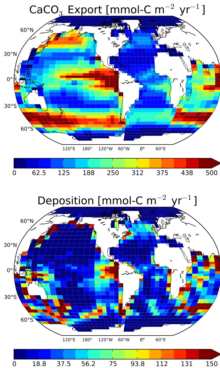
Figure 7. Top: median \text{CaCO}_3 export, globally 0.90 (0.72–1.05) \text{Gt-C yr}^{-1} . Bottom: median \text{CaCO}_3 fluxes reaching the ocean floor, globally 0.164 (0.113–0.227) \text{Gt-C yr}^{-1} . Note the different scaling of the colourbars.
