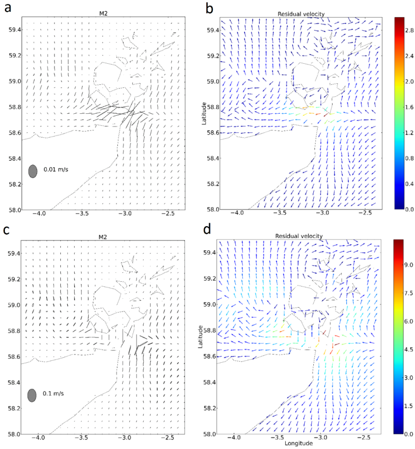
Figure 14. Difference in currents between scenario run and reference run. a) M2 tidal current ellipses and b) residual currents [ \text{cm/s} ] for the 800 MW extraction scenario. c) M2 tidal current ellipses and d) residual currents [ \text{cm/s} ] for the 8 GW extraction scenario.
