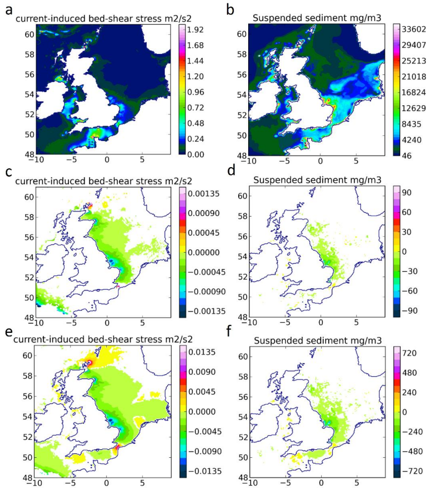
Figure 15. a) annually averaged current-induced bed-shear stress for 2008. b) annually averaged surface SPM concentration for 2008. c) and d): changes in a) and b) for the 800 MW extraction scenario. e) and f): changes in a) and b) for the 8 GW extraction scenario. White areas were masked out.
