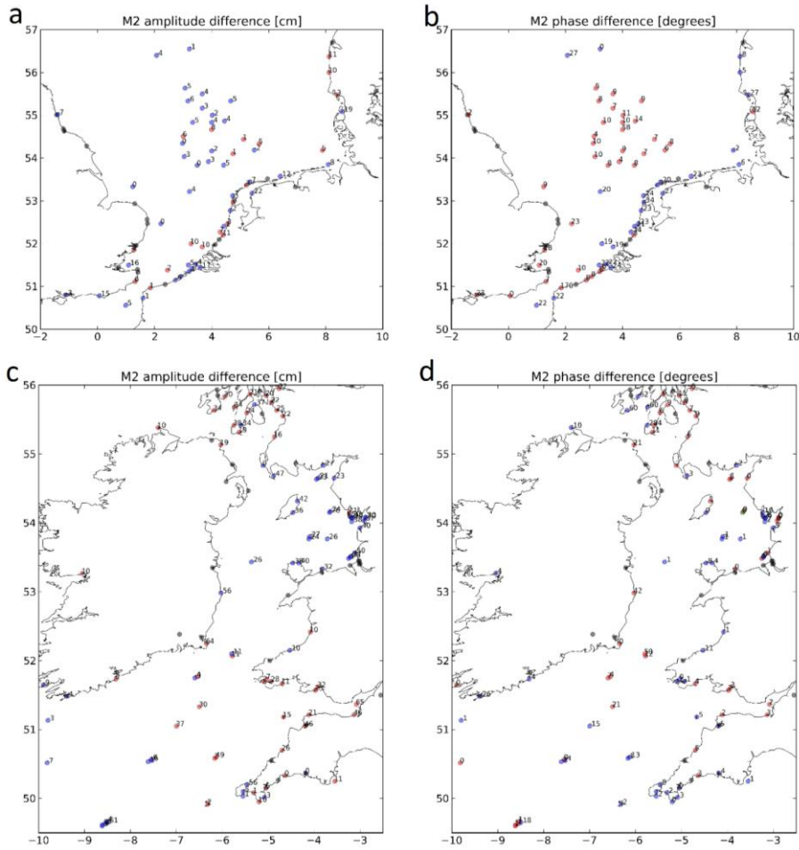
Figure 5. Spatial distribution of difference between model and observations of M2 tidal elevations. a) amplitude and b) phase for the southern North Sea; and c) amplitude and d) phase for the Irish and Celtic Seas. Blue circles: model smaller than observations; red circles: model larger than observations; grey circles: no data, or dry model grid cell at tide gauge location.
