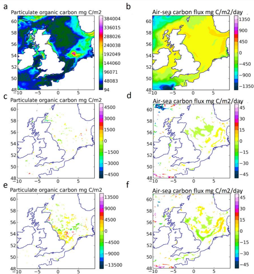
Figure 18. a) annually averaged benthic particulate organic carbon for 2008. b) annually averaged sea-surface CO 2 flux for 2008. c) and d): changes in a) and b) for the 800 MW extraction scenario. e) and f): changes in a) and b) for the 8 GW extraction scenario. White areas were masked out.
