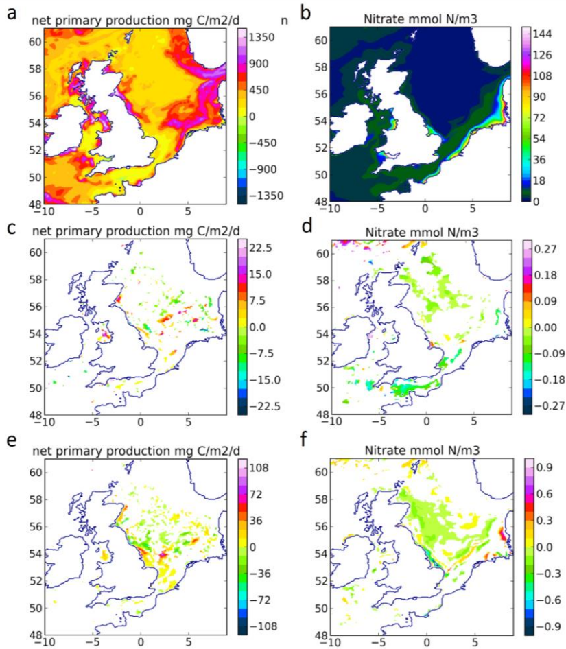
Figure 16. a) annually averaged net primary production for 2008. b) annually averaged surface nitrate concentration for 2008. c) and d): changes in a) and b) for the 800 MW extraction scenario. e) and f): changes in a) and b) for the 8 GW extraction scenario. White areas were masked out.
