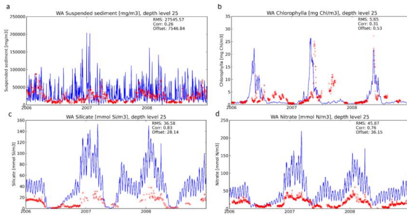
Figure 7. Comparison of model (blue line) with observations (red crosses), for the Warp Anchorage SmartBuoy. a) SPM, b) chlorophyll, c) silicate, d) nitrate.
