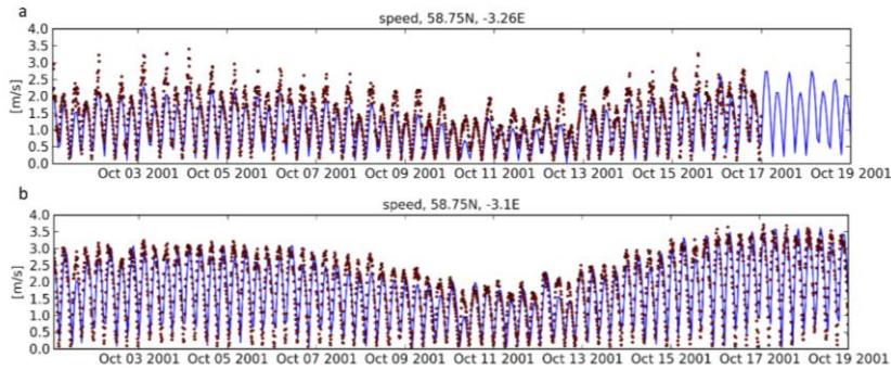
Figure 6. Comparison of modelled tidal current speed in the Pentland Firth with ADCP observations (Gardline Surveys, 2001): a) ADCP 1, b) ADCP 2. Dots: observations, blue line: model results. For locations see Figure 2.
