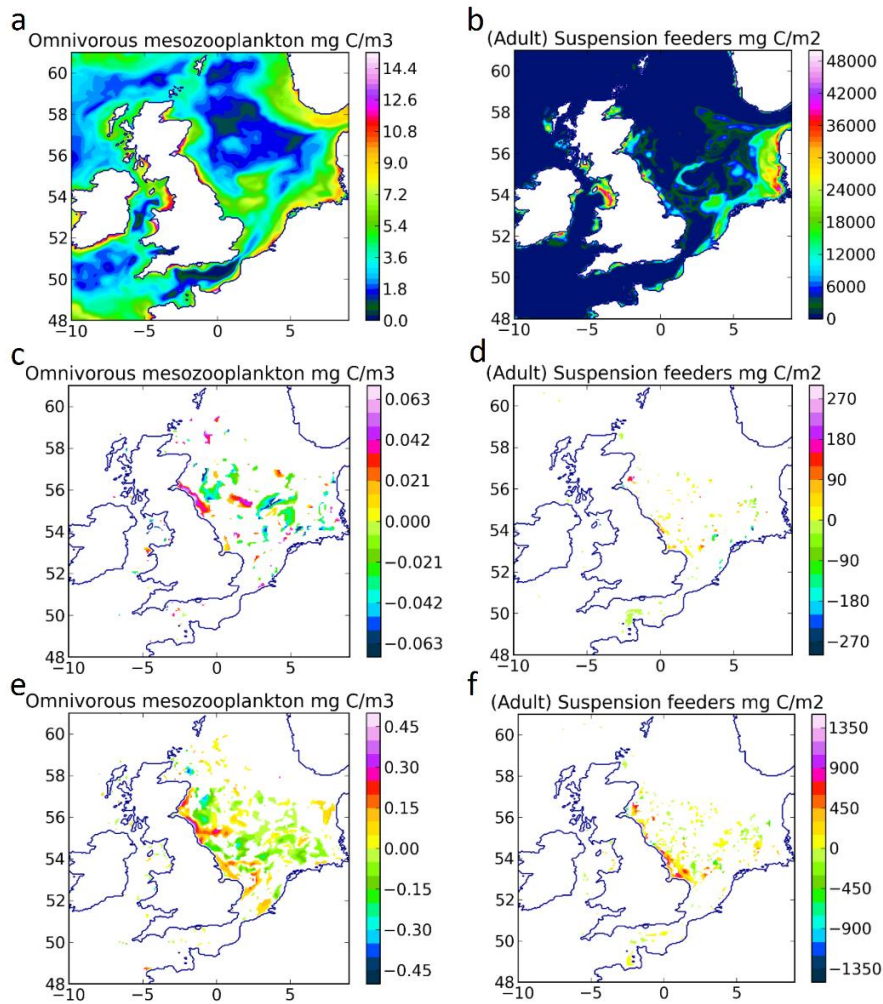
Figure 17. a) annually averaged omnivorous mesozooplankton carbon biomass for 2008. b) annually averaged suspension feeder carbon biomass for 2008. c) and d): changes in a) and b) for the 800 MW extraction scenario. e) and f): changes in a) and b) for the 8 GW extraction scenario. White areas were masked out.
