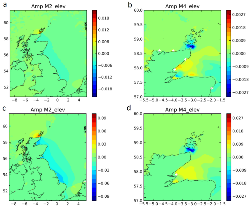
Figure 13. Difference in tidal elevations between scenario run and reference run. a) M2 amplitude [m] and b) M4 amplitude [m] for the 800 MW extraction scenario. c) M2 amplitude [m] and d) M4 amplitude [m] for the 8 GW extraction scenario.
