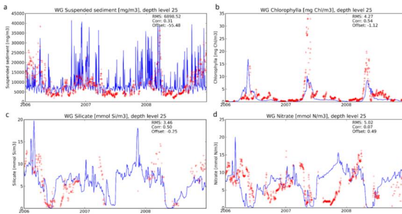
Figure 9. Comparison of model (blue line) with observations (red crosses), for the West Gabbard SmartBuoy. a) SPM, b) chlorophyll, c) silicate, d) nitrate.
