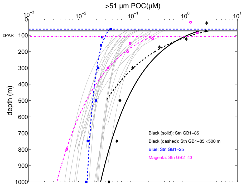
Figure 3. Significant power law fits of > 51 \mu\text{m} [POC] below z_{\text{PAR}} , according to Eq. (1). Only the 22 significant fits are shown as lines. Three stations are highlighted to show the range in > 51 \mu\text{m} [POC] attenuation across GB1 and GB2 profiles (symbols represent measurements): GB1-85 had the highest POC concentration through the water column and an attenuation coefficient of 1.7; GB1-25 had the lowest attenuation coefficient (0.4); GB2-43 had the highest attenuation coefficient (1.9) (Table 2). Fitting GB1-85 > 51 \mu\text{m} [POC] measurements between z_{\text{PAR}} and 500 m yields a higher attenuation coefficient of 2.35. Refer to Fig. 1 for station locations.
