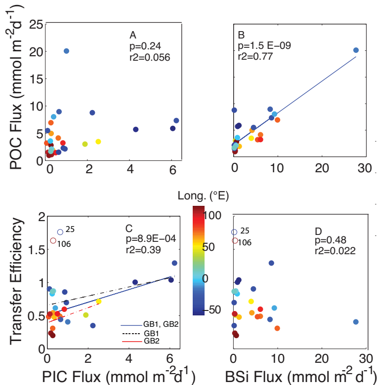
Figure 9. ^{234}\text{Th} -derived POC flux as a function of (a) PIC flux and (b) BSi flux at z_{\text{PAR}} . POC flux transfer efficiency between z_{\text{PAR}} and z_{\text{PAR}} + 100\text{ m} ( T_{100} , defined in Sect. 4.4) as a function of (c) PIC flux and (d) BSi flux at z_{\text{PAR}} . Significant linear relationships are plotted as a solid blue line. T_{100} values at GB1-25 and GB2-106 were excluded from all correlations (Sect. 4.4). Colorbar indicates longitude of stations – GB1 and GB2 stations are in cool and warm colors, respectively. Refer to Fig. 1 for more specific station locations.
