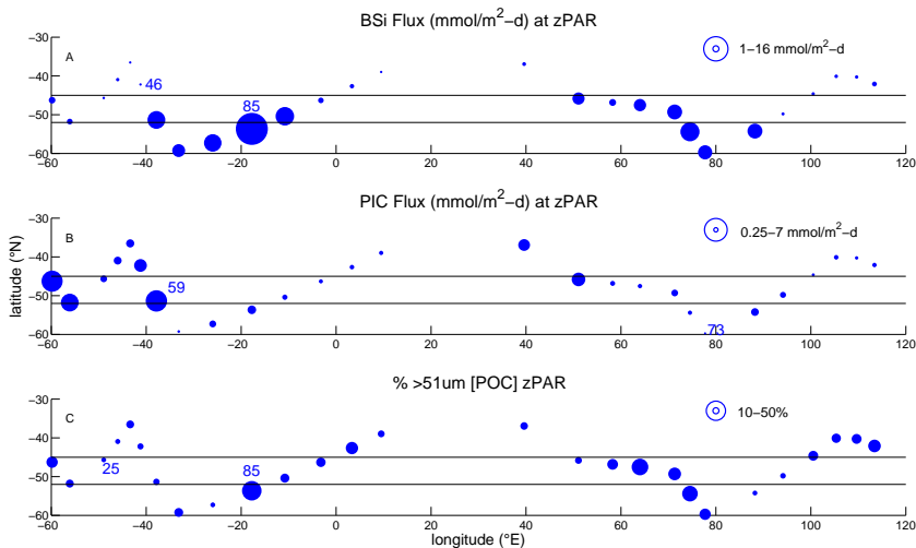
Figure 6. Distribution of BSi flux, PIC flux, and % > 51 \mu\text{m} [POC], the percent of total [POC] in the > 51 \mu\text{m} size class, at z_{\text{PAR}} (Table 1) along GB1 and GB2. (a) BSi fluxes range from 0.17 to 28 \text{mmol m}^{-2} \text{d}^{-1} at stations GB1-46 and GB1-85, respectively. (b) PIC fluxes range from 0.067 to 6.2 \text{mmol m}^{-2} \text{d}^{-1} at stations GB2-73 and GB2-59, respectively. (c) The proportion of [POC] in the > 51 \mu\text{m} size-fraction at z_{\text{PAR}} ranges from 3.3 to 52 % at stations GB1-25 and GB1-85, respectively. A few station numbers discussed in the text are indicated. The two horizontal dashed lines at 45 and 52° S represent the approximate locations of the Subantarctic and Polar fronts, respectively (Belkin and Gordon, 1996; Sokolov and Rintoul, 2009). Refer to Fig. 1 for other station locations.
