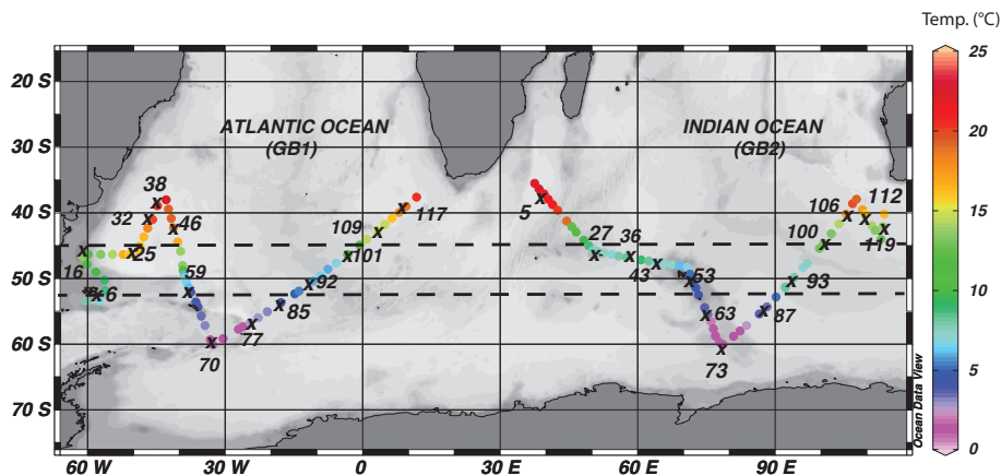
Figure 1. Cruise tracks across the Atlantic (cruise GB1) and Indian (cruise GB2) sectors of the Great Calcite Belt showing sea surface temperature along the two transects. Station numbers where only ^{234}\text{Th} and size-fractionated particles were sampled are indicated by crosses. The two horizontal dashed lines at 45 and 52° S represent the approximate locations of the Subantarctic and Polar fronts, respectively (Belkin and Gordon, 1996; Sokolov and Rintoul, 2009).
