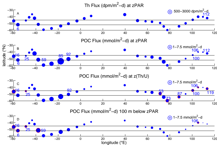
Figure 5. Distribution of ^{234}\text{Th} flux and ^{234}\text{Th} -derived POC flux at 27 stations along GB1 and GB2. (a) ^{234}\text{Th} fluxes at z_{\text{PAR}} range from 717 to 2437 \text{dpm m}^{-2} \text{d}^{-1} at stations GB2-112 and GB1-6, respectively. (b) POC fluxes at z_{\text{PAR}} range from 0.97 to 20 \text{mmol m}^{-2} \text{d}^{-1} at stations GB2-112 and GB1-85, respectively. (c) POC fluxes at z_{\text{Th/U}} range from 0.57 to 12 \text{mmol m}^{-2} \text{d}^{-1} at stations GB2-112 and GB1-85, respectively (Table S2). (d) POC fluxes at 100 m below z_{\text{PAR}} range from 0.23 to 9.5 \text{mmol m}^{-2} \text{d}^{-1} at stations GB2-112 and GB1-59, respectively. A few station numbers discussed in the text are indicated. Red outlines distinguish stations where fluxes are greater at the specified depth than at z_{\text{PAR}} . The two horizontal dashed lines at 45 and 52° S represent the approximate locations of the Subantarctic and Polar fronts, respectively (Belkin and Gordon, 1996; Sokolov and Rintoul, 2009). Refer to Fig. 1 for other station locations. z_{\text{PAR}} and z_{\text{Th/U}} are defined as in Table 1.
