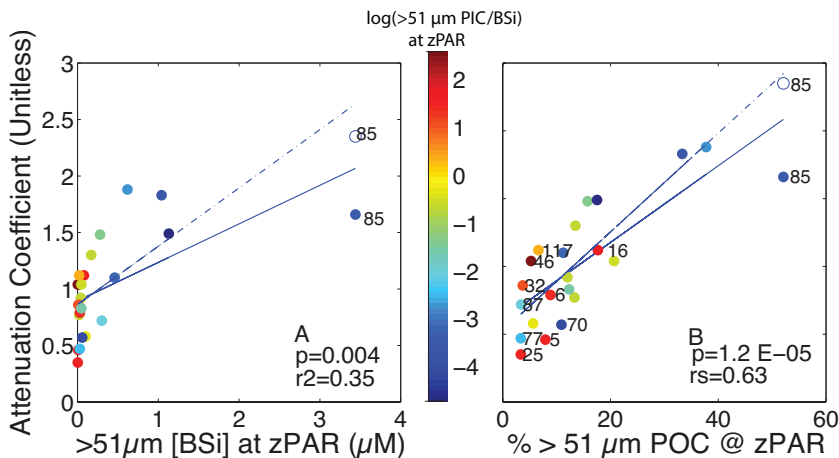
Figure 10. Attenuation coefficient as a function of (a) > 51 \mu\text{m} [BSi] at z_{\text{PAR}} and (b) the proportion of [POC] in the > 51 \mu\text{m} size-fraction at z_{\text{PAR}} . The open circle indicates where GB1-85 would plot with a higher attenuation coefficient of 2.35, derived from fitting > 51 \mu\text{m} [POC] at depths between z_{\text{PAR}} and 500 m. Significant linear relationships using the lower and higher attenuation coefficient values for GB1-85 are shown as solid and dashed lines, respectively; p and r^2 values are provided for the solid lines. The colorbar is the natural logarithm of the ratio of > 51 \mu\text{m} PIC : BSi at z_{\text{PAR}} . We interpret all warm colors > 0 to indicate coccolithophore-dominated stations, and all cool values < 0 to indicate diatom-dominated stations. A few station numbers discussed in the text are indicated. Refer to Fig. 1 for station locations.
