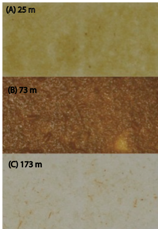
Figure 2. Digital images of > 51 \mu\text{m} filters from station GB1-85 (refer to Fig. 1 for station location). > 51 \mu\text{m} particles are from (a) 25 m in the euphotic zone, (b) 73 m, which corresponds to Z_{\text{PAR}} , as defined in Table 1, and (c) at 173 m, below both metrics of export depth, Z_{\text{PAR}} and Z_{\text{Th/U}} (Table 1). > 51 \mu\text{m} particles appear as intact cells in the euphotic zone (a, b) and as fecal pellets below Z_{\text{PAR}} (c) .
