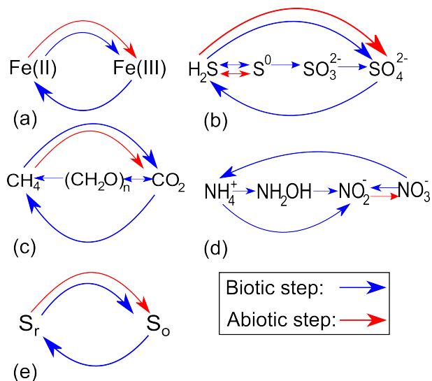
Figure 1. Schematic view of the biogeochemical redox cycles involving iron, sulfur, carbon and nitrogen ( a–d ) (Falkowski et al., 2008; Fenchel et al., 1998; Galloway et al., 2004; Canfield et al., 2005), together with the model investigated in the first part of this work ( e ). In all panels, oxidation reactions proceed to the right, and reduction reactions proceed to the left. Biologically catalysed (metabolic) reactions are shown in blue, and abiotic reactions are shown in red. We note that abiotic reduction reactions are not shown, as these are minor reactions in the natural environment (but can be included in our model, see Supplement, Sect. S1). We also note that many intermediate chemical states are not shown (particularly for the nitrogen and sulfur cycles) but inclusion of extra states does not affect our conclusions; see Supplement. In panel ( e ), s_r and s_o represent the reduced and oxidized forms of the chemical element being cycled.
