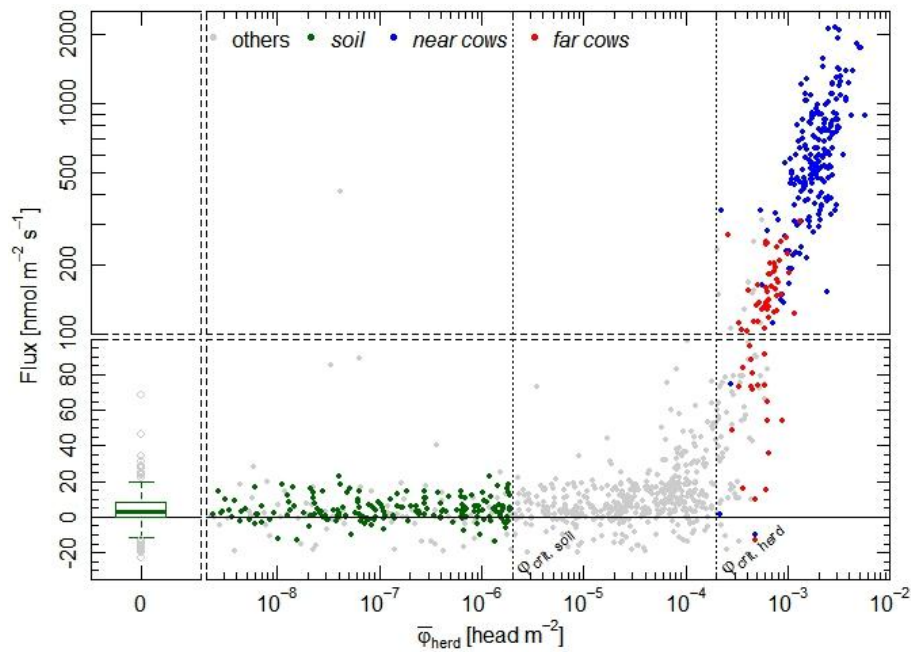
Figure 6. Quality selected 30 min CH 4 fluxes plotted against the mean herd footprint weight ( \bar{\varphi}_{\text{herd}} ). Cases used for soil flux and cow emission calculation are marked in color. Points in gray correspond to selected fluxes before the attribution into soil and cow fluxes and outlier removal.
