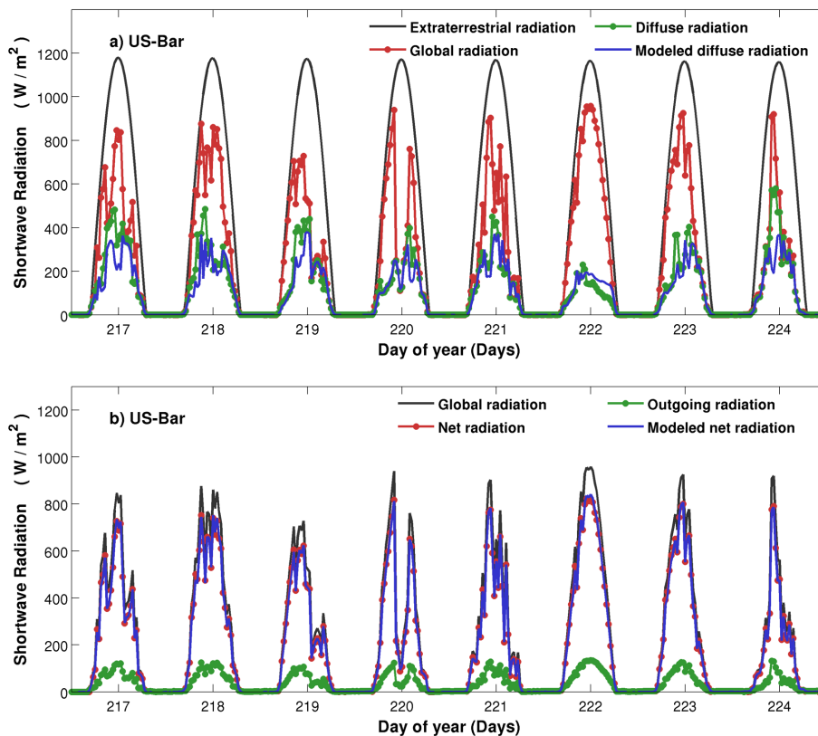
Figure 4. Time series of measured and modeled components of (a) the partition of global solar radiation and (b) surface radiation balance are shown for 8 successive days. Extraterrestrial radiation is derived following methods outlined in Allen et al. (1998). Muneer's method is applied to model diffuse radiation. The GORT model is applied to model net radiation. Data are shown from the Day of Year 217 to 224 in 2004 for the US-Bar site.
