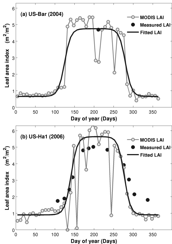
Figure 8. Comparisons of field-measured and satellite-derived leaf area indexes (LAI) for the sites (a) US-Bar in 2004 and (b) US-Ha1 in 2006. The solid grey lines denote MODIS LAI as obtained from standard MODIS FPAR/LAI products (MOD15A2). The solid black lines denote double logistic fitting lines that are applied to MODIS LAI. The solid points denote the measured LAI as obtained from biological datasets from AmeriFlux website.
