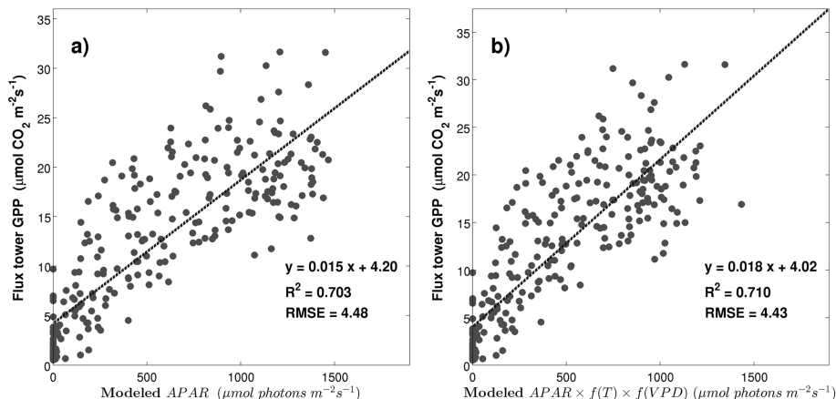
Figure 12. Regressions between modeled absorbed photosynthetic active radiation (APAR) and measured GPP. Half-hourly data are shown from DOY 217–224 in 2004 for US-Bar. The influences of temperature and vapor pressure deficit are modeled based on Eqs. (51) and (52). Only data during the photosynthetically active period are included in the regression. The dashed lines denote the regression lines.
