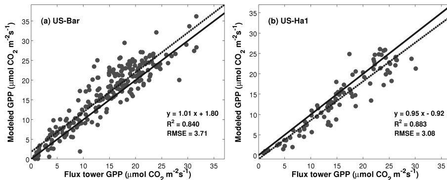
Figure 7. Regressions between modeled and measured GPP for 8 consecutive days at the sites (a) US-Bar and (b) US-Ha1. Data are from DOY 217–224 in 2004 for US-Bar and from DOY 241 to 224 in 2006 for US-Ha1. Only data during the photosynthetically active period (flux tower GPP > 0.5 \mu\text{mol CO}_2 \text{ m}^{-2} \text{ s}^{-1} ) are included in the regression. The solid lines denote the 1 : 1 lines, and the dashed lines denote the regression lines.
