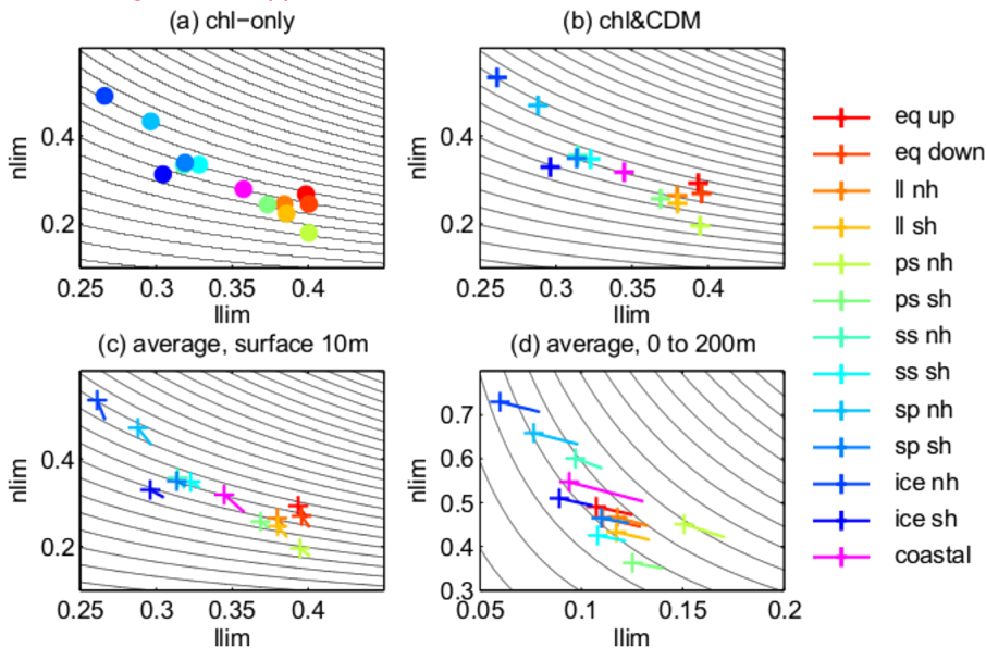
Figure 14. Light and nutrient limitation scaling factors for open ocean biomes and coastal regions. (a) Average n_{lim} , l_{lim} for chl-only model run, from 0 to 10 m (b) average n_{lim} , l_{lim} for chl&CDM model run, from 0 to 10 m (c) vectors connecting coordinates from panel (a, b) , average from 0 to 10 m. (d) Vectors starting at coordinates from chl-only model run and terminating with an “x” at values from chl&CDM model run, average from 0 to 200 m. Legend abbreviations: ice = marginal ice zone, sp = subpolar, ss = seasonally stratified, ps = permanently stratified, ll = lower latitude, eq up = equatorial upwelling, eq down = equatorial downwelling, coastal = coastal regions, defined as the grid cells adjacent to land. Suffixes nh and sh stand for Northern Hemisphere and Southern Hemisphere.
