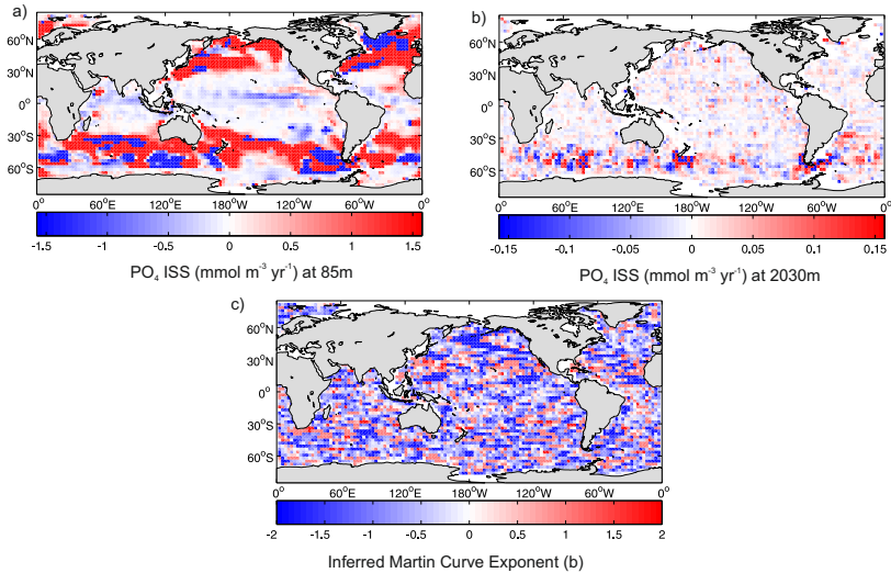
Figure 2. Example of using a GCM transport matrix to estimate \text{PO}_4 remineralisation rates. (a) The estimated \text{PO}_4 remineralisation rates generated using the MIT GCM transport matrix at 85 m and (b) 2030 m. (c) Power law flux curve exponents (b) inferred from the estimated remineralisation rates by fitting a linear function to the log transformed data as in Fig. 1b.
