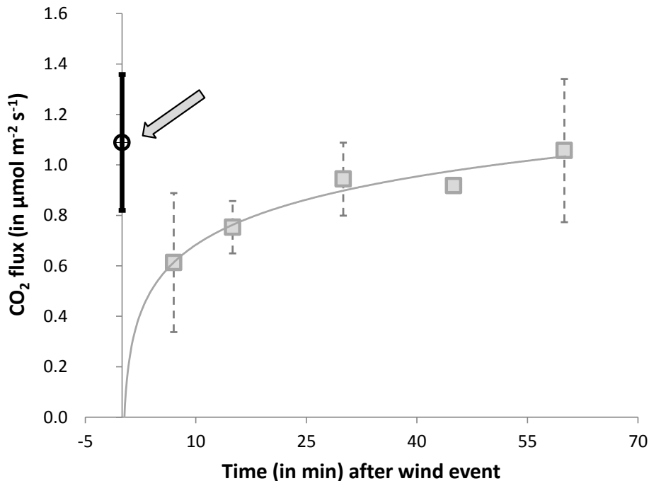
Figure 5. Flux recovery from peat soils after high wind events. Open circle (o) represents fluxes taken under zero wind conditions prior to wind events. Gray closed squares represent fluxes measured under zero wind conditions after wind events. The logarithmic trend line indicates best fit to data ( y = 0.195 \times \ln(t(\text{min})) + 0.233 ; r^2 = 0.95 ). Error bars indicate SD; n \geq 3 .
