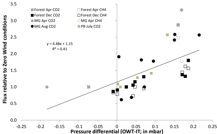
Figure 4. The relationship between measured pressure differential (outer wind tunnel minus inner toroid, in mbar) and flux relative to zero wind conditions ( F_R ). For direct comparison, only data included in Fig. 3 have been included in this figure. Solid fill symbols indicate CO 2 flux ratios while open symbols show CH 4 flux ratios (Tables 2, 3). Trend line indicates best fit for data ( r^2 = 0.41 , y = 4.48 \times \text{Pressure differential (mbar)} + 1.15 ).
