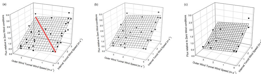
Figure 3. (a) Relationship between wind speeds internal and external to the toroid and relative fluxes for the pooled CO 2 ( n = 27 ) and CH 4 ( n = 13 ). Planar surface indicates best fit to data ( z = 0.98 + 0.54 \times \text{IT WS} - 0.11 \times \text{OWT WS} ; r^2 = 0.82 ). The shaded red line represents equal wind speeds inside and outside the flux chamber, where z = 0.098 + 0.42 \times \text{IT/OWT WS} ( \text{m s}^{-1} ). (b) and (c) show disaggregated CO 2 and CH 4 data, with (b) showing the relationship between wind speeds internal and external to the toroid and relative CO 2 fluxes ( n = 27 ). All details as shown in Fig. 3a. Planar surface indicates best fit to data ( z = 1.021 + 0.57 \times \text{IT WS} - 0.13 \times \text{OWT WS} ; r^2 = 0.85 ). For (c) we show the relationship between wind speeds internal and external to the toroid and relative CH 4 fluxes ( n = 13 ). All details as shown in Fig. 3a. Planar surface indicates best fit to data ( z = 0.94 + 0.43 \times \text{Internal WS} - 0.09 \times \text{External WS} ; r^2 = 0.80 ).
