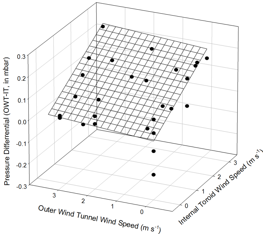
Figure 2. The relationship between wind speed and measured pressure differential (outer wind tunnel minus inner toroid). The planar surface indicates best fit to data ( r^2 = 0.63 , z = -0.03 + 0.07 \times \text{IT WS (m s}^{-1}) + 0.01 \times \text{OWT WS (m s}^{-1}) ). Note insensitivity of pressure to external wind speeds.
