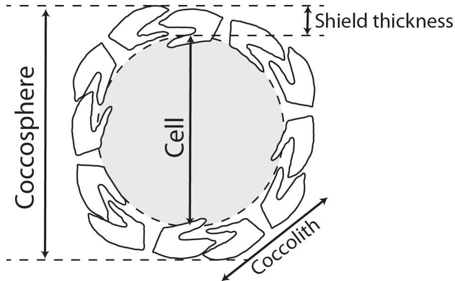
Figure 1. Schematic representation of a coccolithophore cell surrounded by a shield of coccoliths. The coccolith bearing-cell is called the coccosphere (modified from Hendericks, 2008).
