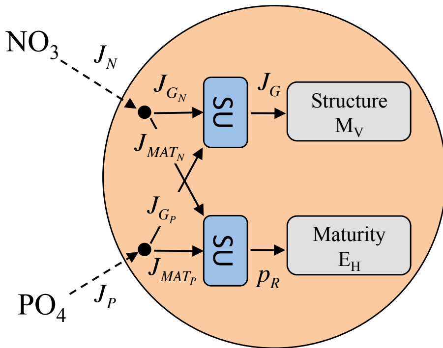
Figure 9. Simple physiological model of a dividing phytoplankton cell that reproduces the co-variation of metabolic rates and cell-size observed in coccolithophores. Notes: J_X – assimilation fluxes; J_{GX} – growth fluxes generated from the uptake of nutrient X ; J_{MATX} – maturation fluxes generated from the uptake of nutrient X ; J_G – total growth flux contributing to the buildup of structure (biomass) M_V ; p_R – total maturation flux contributing to the buildup of maturity E_H ; SU – synthesizing unit.
