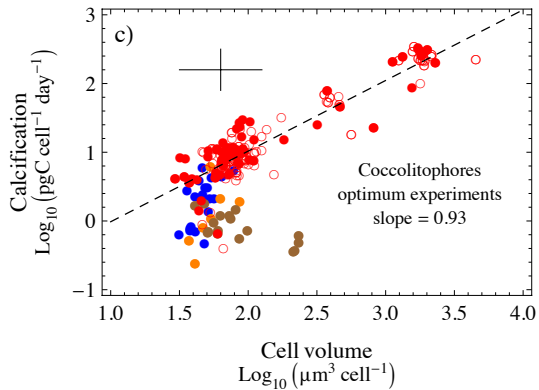
Figure 4. Effect of sub-optimum growth conditions on allometric relationships for coccolithophores. (a) Rate of photosynthesis, (b) growth rate, (c) rate of calcification. Sub-optimum light and nutrient conditions result in cells having reduced metabolic rates compared to cells of equal size grown in optimal growth conditions (see Table 2 for definition of growth conditions). The error bars apply only to a limited number of experiments (see text) and correspond to those experiments where the sampling time is not reported.
