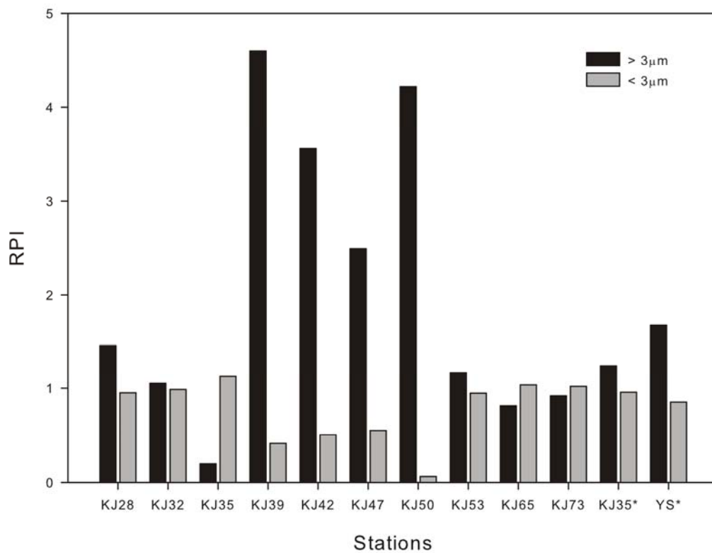
2 Figure 4. Relative preference index (RPI) for size-fractionated phytoplankton. > 3 µm, size 3 fraction larger than 3 µm; < 3 µm, size fraction smaller than 3 µm; the asterisk indicates 4 experiments conducted in May 2009, others were conducted in November 2010. RPI > 1 5 indicates positive selection and vice versa.
