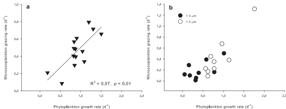
Figure 4. Correlation between phytoplankton growth and microzooplankton grazing rates. (a) May to June 2009; (b) November 2010; > 3 μm, size fraction larger than 3 μm; < 3 μm, size fraction smaller than 3 μm.
