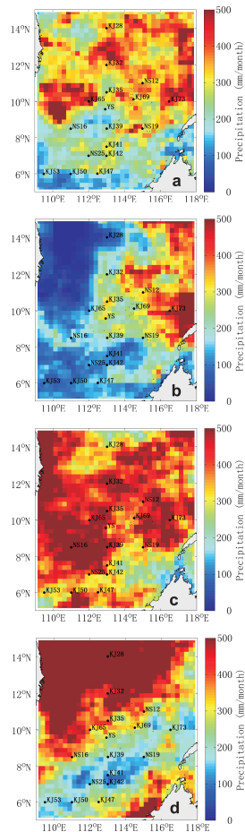
Figure 5. Monthly rainfall in the southern South China Sea estimated on the basis of data from the Tropical Rainfall Measuring Mission. (a) May 2009; (b) June 2009; (c) October 2010; (d) November 2010.
