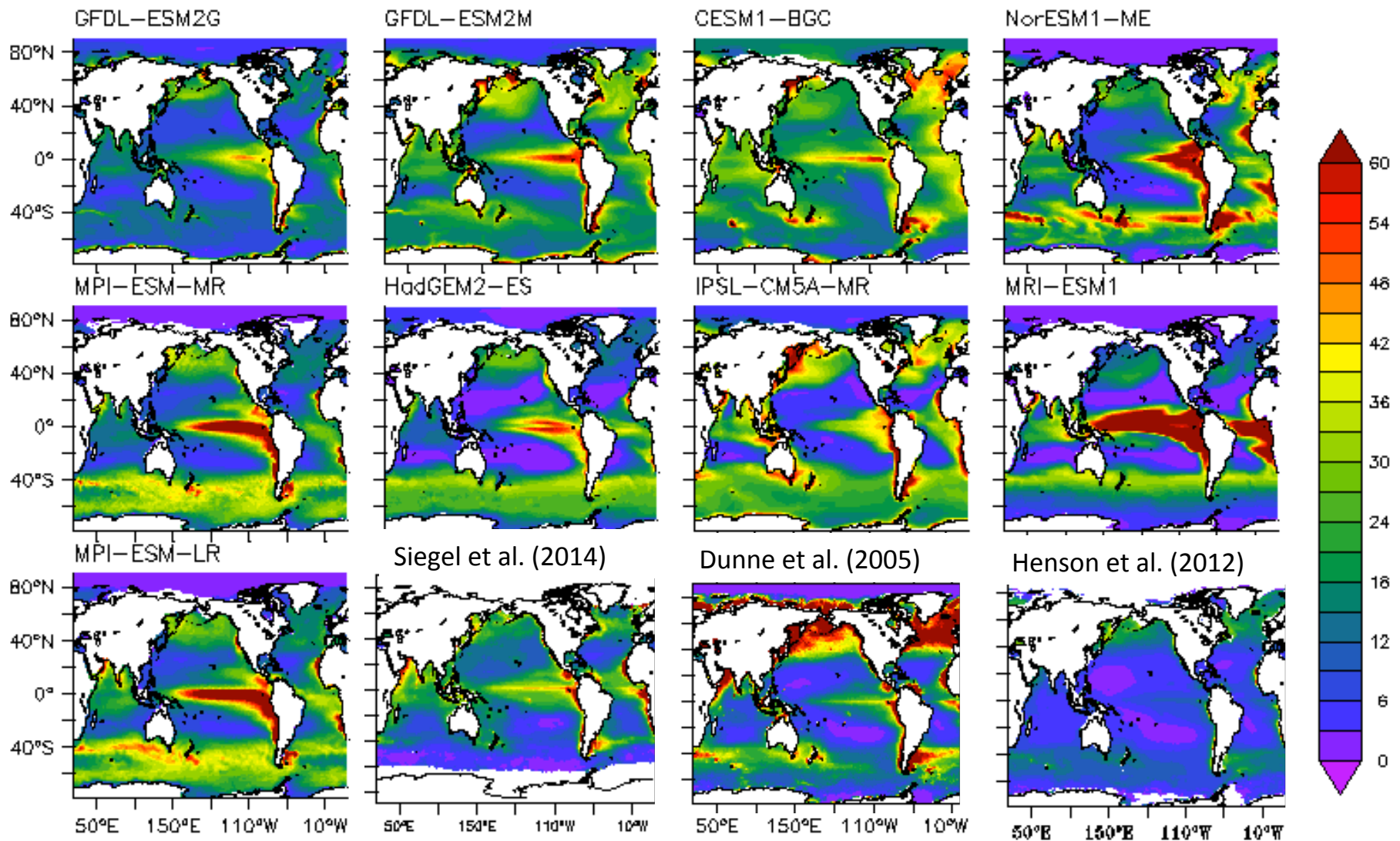
Figure S1: POC flux at 100m [ \text{gC}/\text{m}^2/\text{yr} ] across CMIP5 models. Last three panels show POC flux in the euphotic layer derived from satellite measurements in Siegel et al. (2014), Dunne et al. (2005) and Henson et al. (2012).
