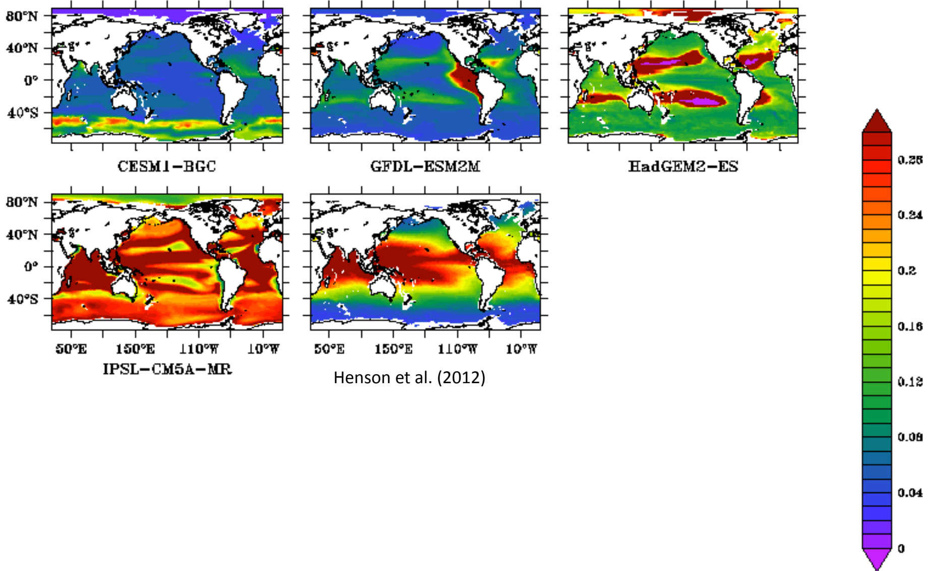
Figure S2: Transfer efficiency of POC flux from 100 m to 2000 m (POC flux at 2000m divided by POC flux at 100m) across the four CMIP5 models that provided a complete depth profile for POC. Last panel shows satellite-derived results from Henson et al. (2012). Note huge variation across CMIP5 models.
