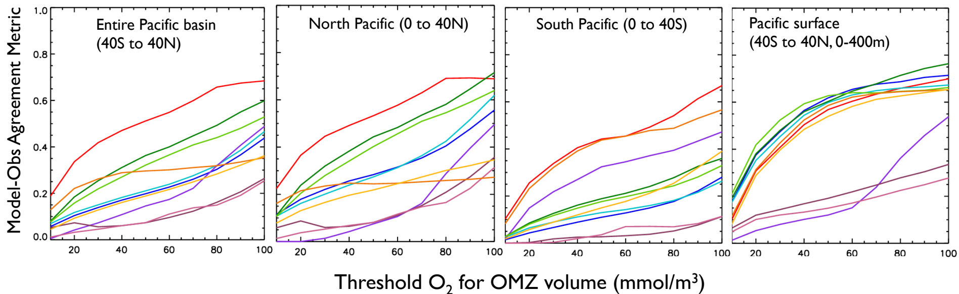
Figure S3: Model performance compared to observations in different regions and depths in the Pacific during the historical period (1960-1999). a)-d) Agreement between OMZ in models and observations described as the intersection of modeled and observed OMZ volumes divided by the union of modeled and observed OMZ volumes at different O_2 thresholds (x axis) and in different regions as labeled. Color bars as in Fig. 7.
