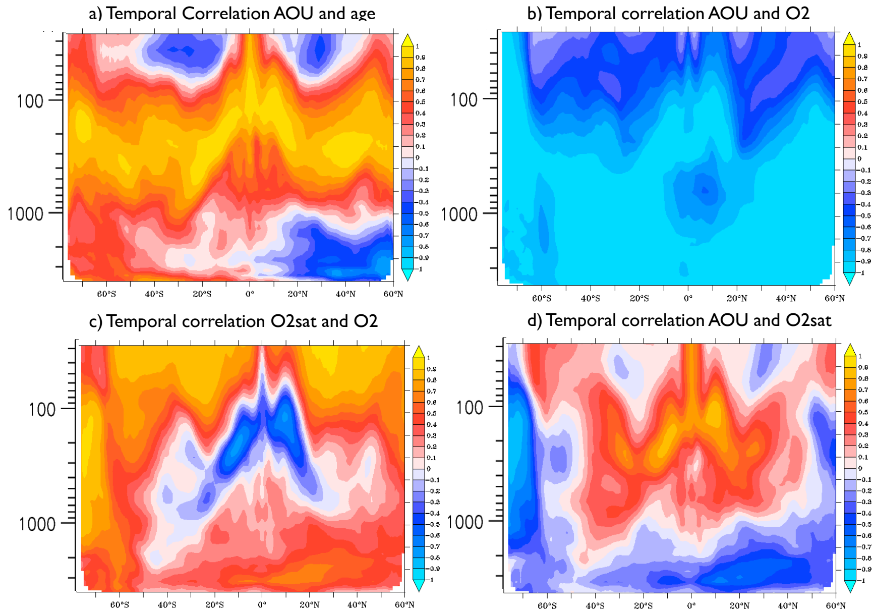
Figure S7: Interannual correlations calculated in a 100-year long control sample (“piControl” scenario). We show the multi-model average across all the available CMIP5 models.
