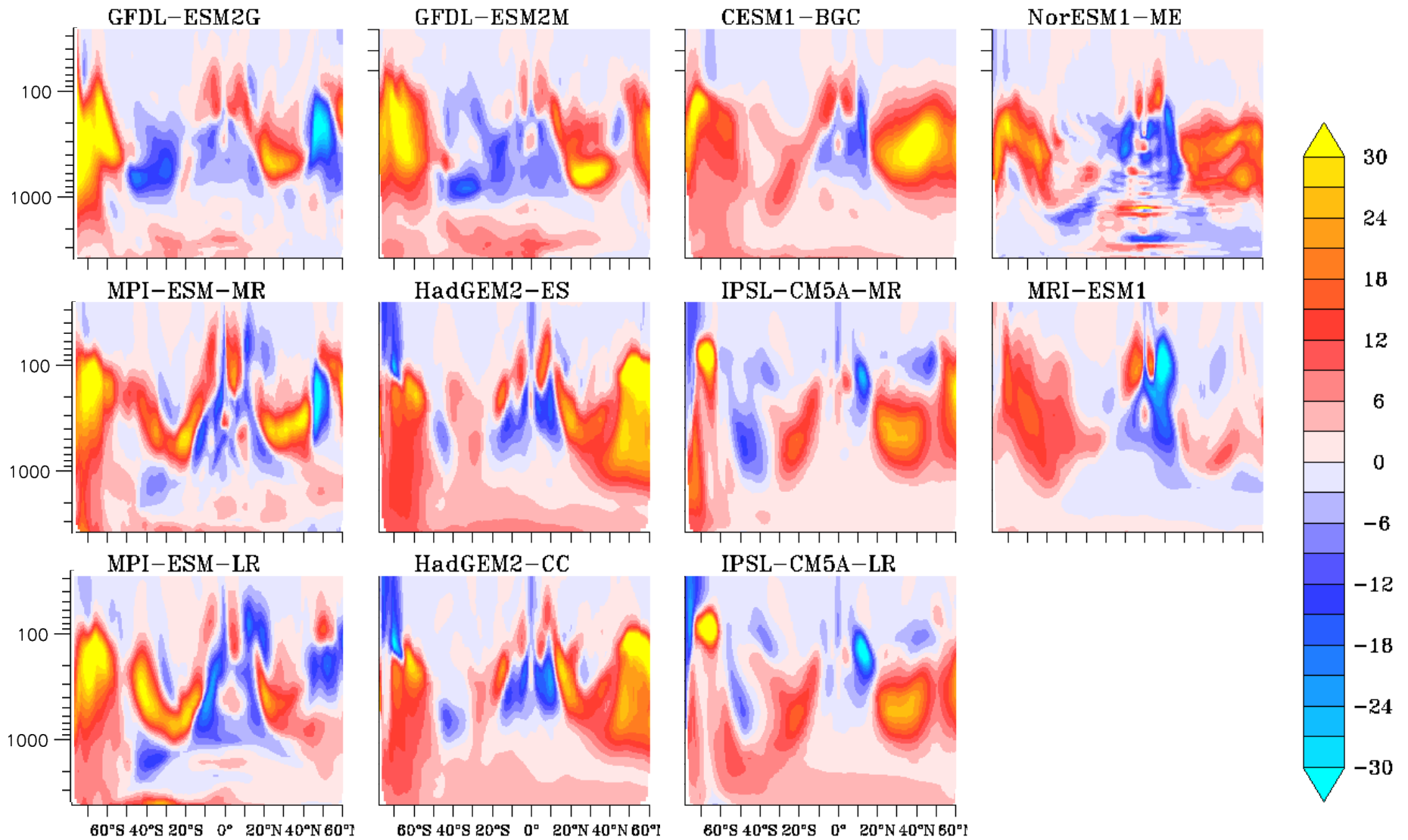
Figure S5: CMIP5 future projections for the period 2060-2099 with reference to the historical period (1960-1999) for AOU ( \text{mmol}/\text{m}^3 ) all averaged zonally between 180^\circ\text{W} and 100^\circ\text{W} in the Pacific Ocean (complementary to Fig. 8f).
