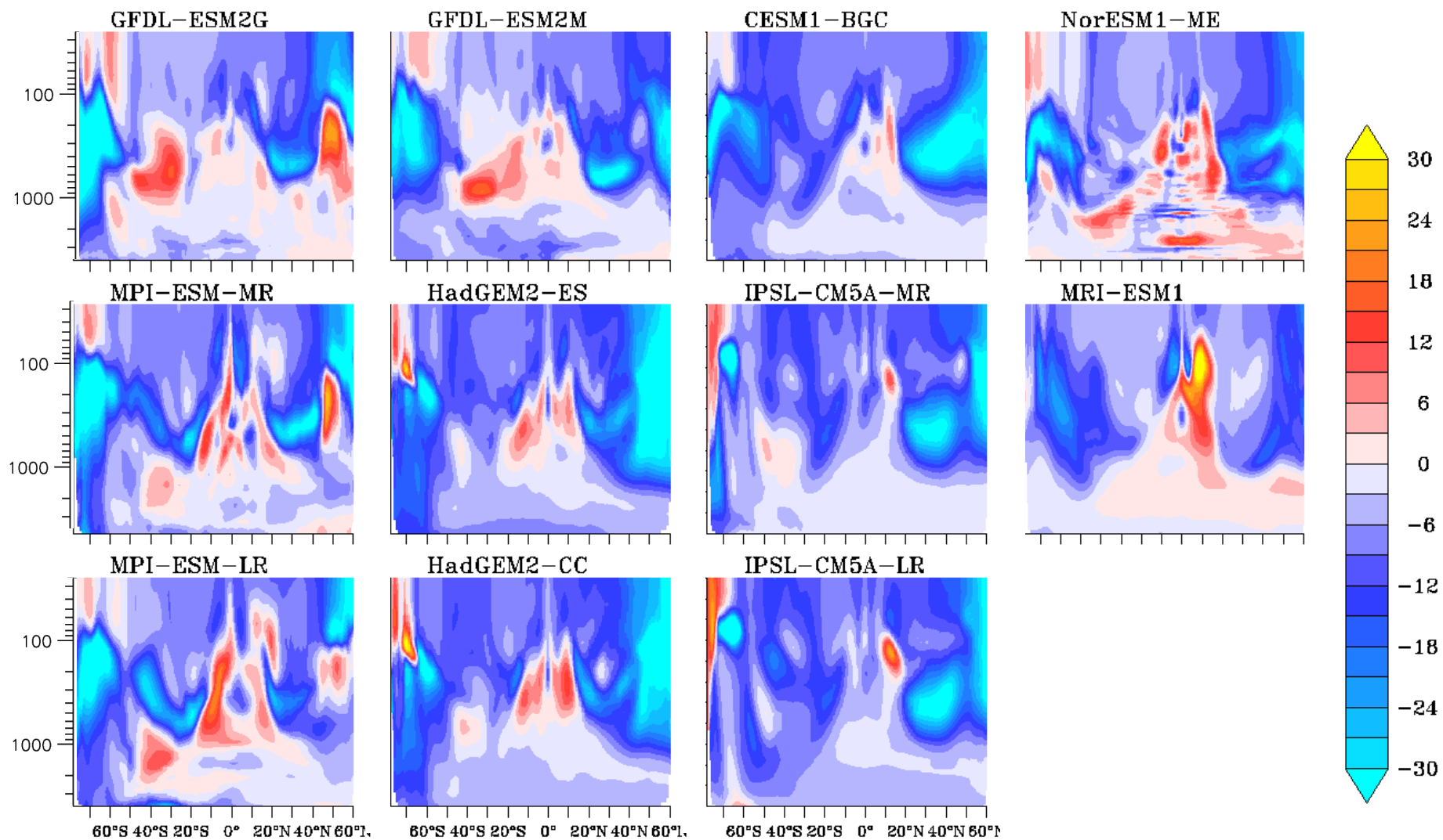
Figure S4: CMIP5 future projections for the period 2060-2099 with reference to the historical period (1960-1999) for oxygen concentration ( \text{mmol/m}^3 ) all averaged zonally between 180^\circ\text{W} and 100^\circ\text{W} in the Pacific Ocean (complementary to Fig. 8c).
