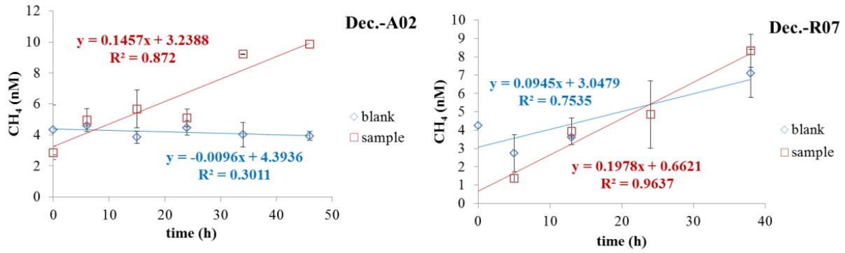
Fig. S1 Variation of CH 4 concentration with time during sediment incubation experiments (Square: overlying water; diamond: control)
