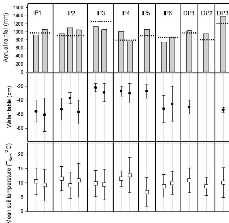
Figure 1. Annual rainfall, mean annual water tables, mean annual temperature at 5 cm depths ( T_{5\text{cm}} ) at sites IP1 (two years), IP2 (three years), IP3 (two years), IP4 (two years), IP5 (one year), IP6 (two years), DP1 (one year), DP2 (one year) and DP3 (one year). Dotted horizontal line indicates 30 year mean rainfall at each site (1981–2010; Met Éireann http://www.met.ie/ and Met Office UK; http://www.metoffice.gov.uk ). Error bars are SDs. Negative water table values indicate water level below the soil surface.
