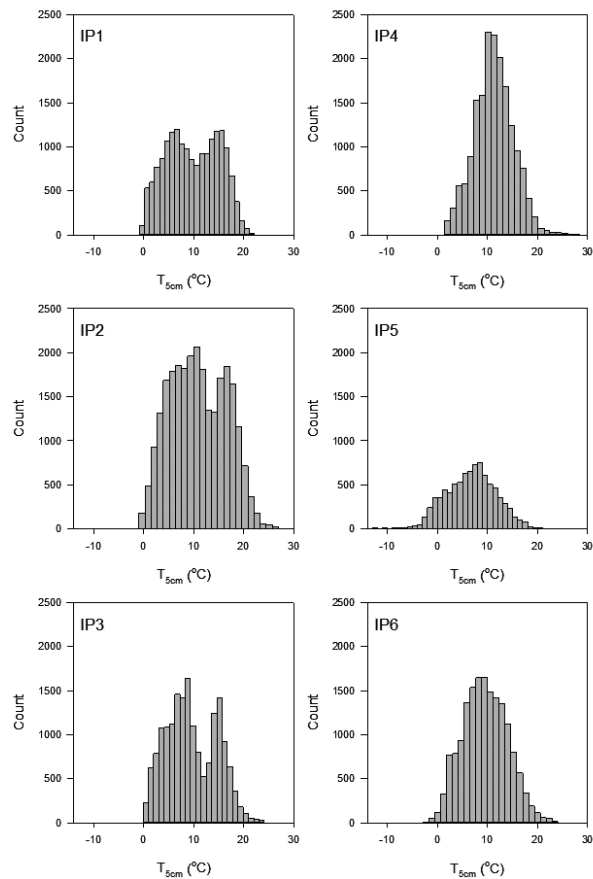
Figure 2. Frequency distribution of soil temperature at 5 cm depth ( T_{5cm} ) at sites IP1–6.
