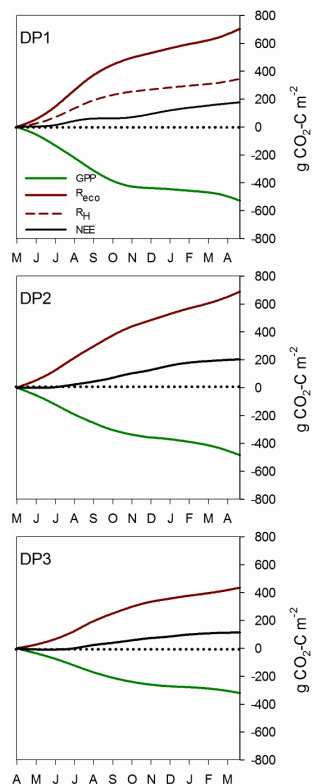
Figure 5. Annual cumulative gross primary productivity (GPP: \text{g CO}_2\text{-C m}^{-2} ), ecosystem respiration ( R_{\text{eco}} : \text{g CO}_2\text{-C m}^{-2} ), heterotrophic respiration ( R_{\text{H}} : site DP1 only) and net ecosystem exchange (NEE: \text{g CO}_2\text{-C m}^{-2} ) at sites DP1–3. Positive values indicate \text{CO}_2\text{-C} flux from the peatland to the atmosphere (source) and negative values indicate \text{CO}_2\text{-C} flux from the atmosphere to the peatland (sink). Value at end of the curve indicates the total annual value for each component. Note the differences in integration period between sites (x axis).
