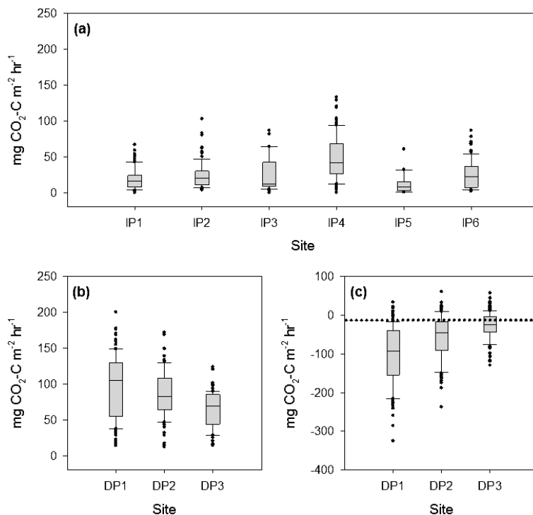
Figure 3. (a) Ecosystem respiration ( R_{\text{eco}} ; \text{mgCO}_2\text{-C m}^{-2}\text{ h}^{-1} ) at sites IP1-6, (b) R_{\text{eco}} ( \text{mgCO}_2\text{-C m}^{-2}\text{ h}^{-1} ) at sites DP1-3 and (c) net ecosystem exchange (NEE; \text{mgCO}_2\text{-C m}^{-2}\text{ h}^{-1} ) at sites DP1-3. Positive values indicate CO 2 -C flux from the peatland to the atmosphere (source) and negative values indicate CO 2 -C flux from the atmosphere to the peatland (sink). The 10th and 90th percentile are indicated by the bars, the 25th and 75th percentiles with the top and bottom of the box and the median value by the centre line. Different letters indicate significant differences in the post-hoc test for multiple comparisons.
