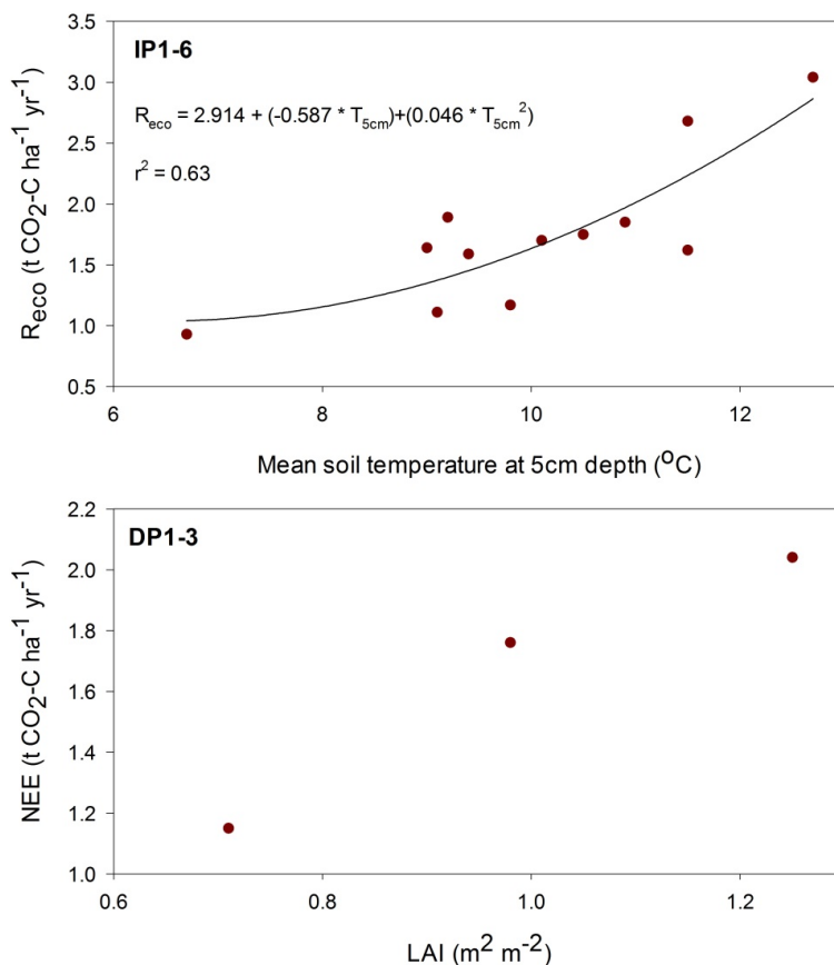
Figure 6. Relationship between (a) ecosystem respiration ( R_{\text{eco}} : tCO 2 -C ha -1 yr -1 ) and mean soil temperature (°C) at 5 cm depth at the IP sites and (b) net ecosystem exchange (NEE: tCO 2 -C ha -1 yr -1 ) and leaf area index (LAI: m 2 m -2 ). Circles indicate an annual value.
