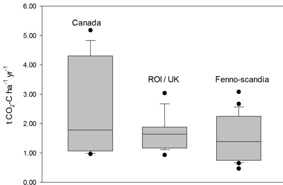
Figure 7. Carbon dioxide emissions ( \text{tCO}_2\text{-C ha}^{-1} \text{yr}^{-1} ) from peatlands managed for extraction in Canada, ROI/UK (this study) and Fenno-scandinavia. The 10th and 90th percentile are indicated by the bars, the 25th and 75th percentiles with the top and bottom of the box and the median value by the centre line (Data for Canada and Fenno-Scandia taken from the following studies; Tuittila and Komulainen, 1995; Sundh et al., 2000; Waddington et al., 2002; Glatzel et al., 2003; McNeil and Waddington, 2003; Tuittila et al., 2004; Cleary et al., 2005; Alm et al., 2007a; Shurpali et al., 2008; Waddington et al., 2010; Järveoja et al., 2012; Mander et al., 2012; Salm et al., 2012; Strack et al., 2014.).
