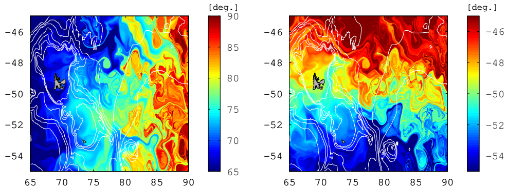
Figure 5. Altimetry-derived 30 days horizontal origin. Left: longitude. Right: latitude.
