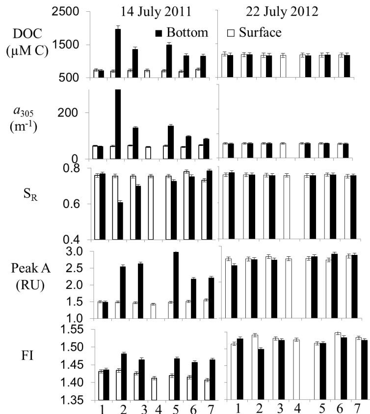
Figure 5. Concentration and quality of DOM in the surface (open bars) and bottom waters (filled bars) in pools 1–7 in Innavait Creek under stratified (left) and mixed (right) conditions in 2011 and 2012, respectively. CDOM and FDOM concentrations shown as absorption coefficients at 305 nm ( a_{305} ) and emission intensities at Peak A (Raman Units; RU), respectively. DOM quality shown as slope ratio ( S_R ) and fluorescence index (FI); CDOM and FDOM proxies for DOM described in text.
