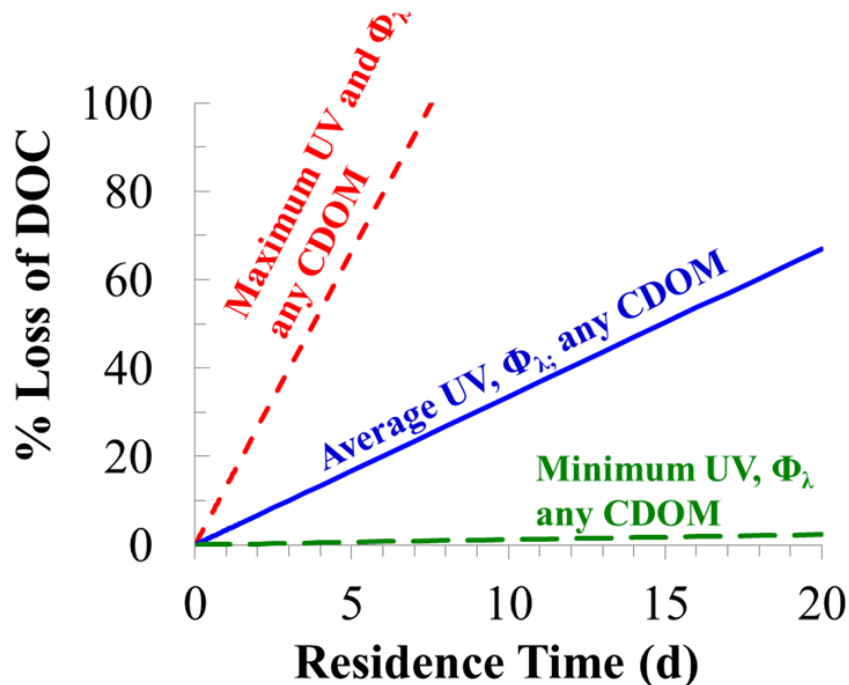
Figure 9. Cumulative percent of DOM concentration loss in Imnavait Creek lost through photo-mineralization as calculated from Eq. (3) (removal of DOC as \text{mol C m}^{-2} \text{d}^{-1} over the mean depth in Imnavait Creek; 0.5 m) in Imnavait Creek using combinations of the range of surface UV light exposure, CDOM concentrations, and apparent quantum yields ( \Phi_\lambda ) measured in this study for up to a 20 day residence time. For each scenario, the initial DOC concentration was set to 943 \mu\text{M C} , the average surface water DOC concentration over both 2011 and 2012 (Table 2). Calculations do not include (1) the effect of DOC loss on changing light attenuation ( K_d ) over the residence time (i.e., CDOM and thus K_{d,\lambda} remain constant over the residence time for each scenario), or (2) the effect of UV light exposure on \Phi_\lambda over time ( \Phi_\lambda , or DOM lability, remained constant over the residence time for each scenario).
