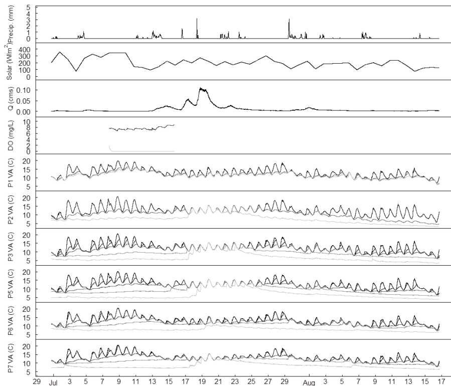
Figure 3. Imnavait Creek precipitation, solar radiation, discharge (at location downstream of study reach), dissolved oxygen in pool 2 top and bottom, and vertical arrays (VA) of temperature sensors within each study pool (P) in summer 2011. The darkest lines represent the sensor at the top of the water column; subsequent lines become lighter with depth of each sensor.
