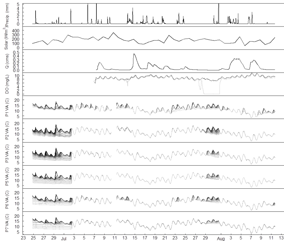
Figure 4. Innavaik Creek precipitation, solar radiation, discharge (at location downstream of study reach), dissolved oxygen in pool 2 top and bottom, and vertical arrays (VA) of temperature sensors within each study pool (P) in summer 2012. The darkest lines represent the sensor at the top of the water column; subsequent lines become lighter with depth of each sensor.
