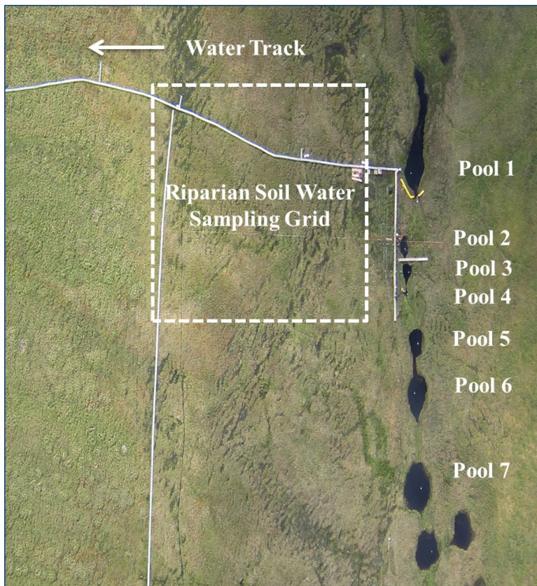
Figure 1. Study area showing the 120 m reach of Imnavait Creek containing seven consecutive pools, and the locations of soil water collection (riparian zone and water track; only the bottom portion of the water track is shown in this image). Also visible in this areal image as white solid lines are boardwalks installed to access sampling sites.
