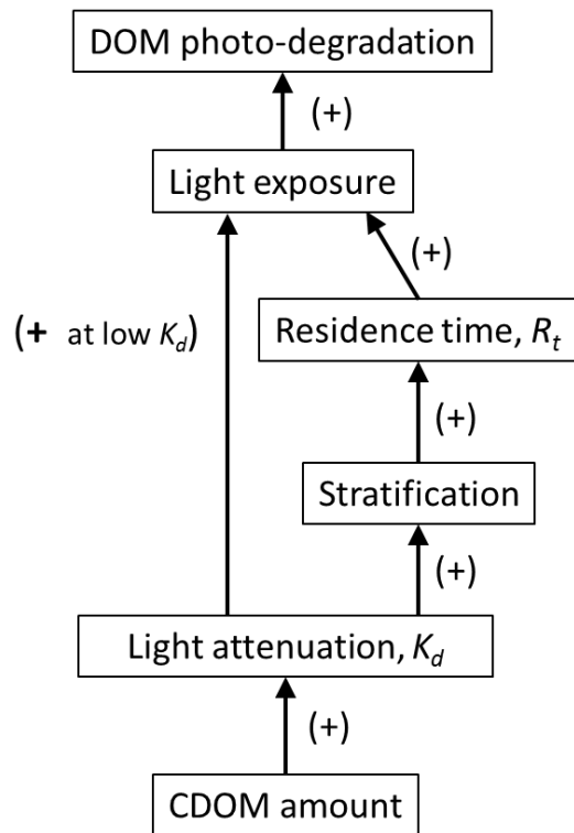
Figure 6. Conceptual diagram illustrating the controls on DOM photo-degradation. As CDOM increases it absorbs more light at the surface and strengthens stratification, which increases residence times, length of light exposure, and thus DOM photo-degradation (right side). Similarly, as CDOM and thus light attenuation increase the total amount of light exposure and light absorption increases in situations where there is low K_d or shallow water column depth z . However, as K_d or shallow water column depth increase the system becomes light limited, and further increases in CDOM result in no change in DOM photo-degradation (asymptote of Fig. S1).
