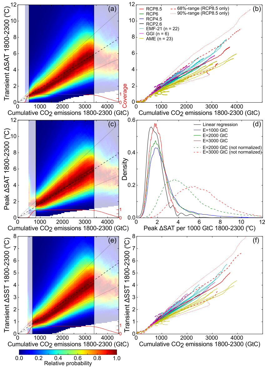
Figure 3. Transient and peak warming as function of cumulative emissions: (a) relative probability of transient surface air temperature change ( \Delta SAT) for given cumulative CO 2 emissions (fossil fuel and deforestation), derived from annual values from ensemble model simulations for 55 greenhouse-gas emission scenarios. Black dashed lines show the median and 68 %-range of the linear regression slope. The red line indicates the coverage of the emission range by the model ensemble. High and low emission ranges with a coverage of less than 90 % are shaded and considered not robust. (b) Transient \Delta SAT response (ensemble median) for the 55 different scenarios. The dashed/dotted lines show the 68/90 %-range of the ensemble for the RCP8.5 scenario, to indicate the model-spread. Please note that our extensions of the RCP scenarios beyond 2100 are not identical to the Extended Concentration Pathways (ECP, see Methods). (c) Same as (a) but for the peak warming for given total cumulative emissions. (d) PDFs of the peak warming for 1000 (blue), 2000 (green), and 3000 GtC (red) cumulative emissions, and for the linear regression (black). The dashed lines indicate the unscaled PDFs and solid lines the normalized response per 1000 GtC. (e, f) Same as (a, b) but for transient sea surface temperature change ( \Delta SST).
