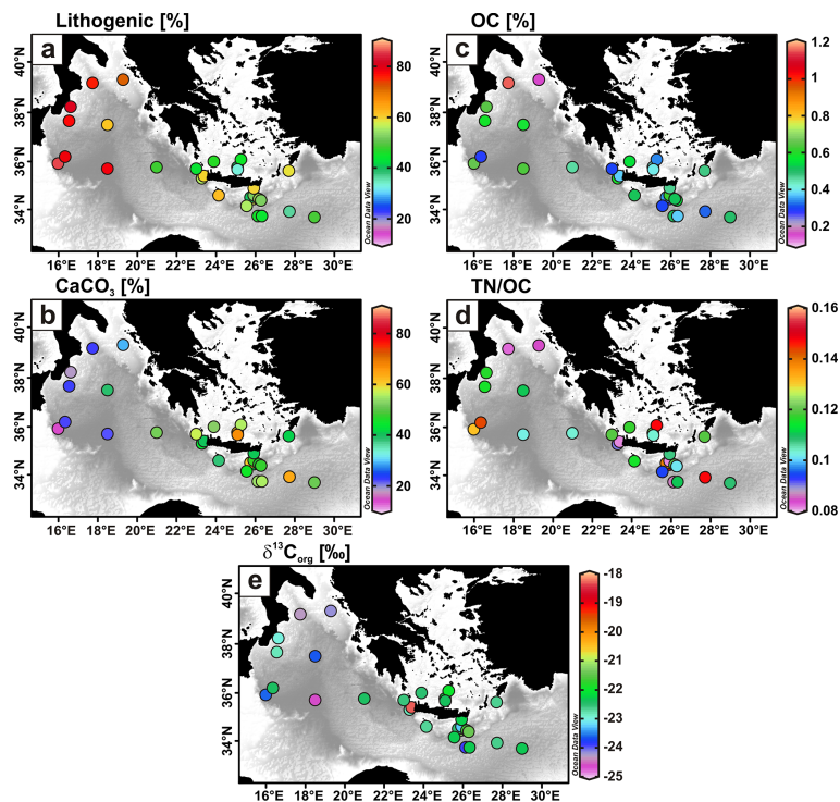
Figure 3. Spatial distribution of (a) lithogenics, (b) CaCO 3 contents, (c) OC contents, (d) TN/OC ratios, (e) and \delta^{13}\text{C} values in surface sediments of the deep Eastern Mediterranean Sea.
