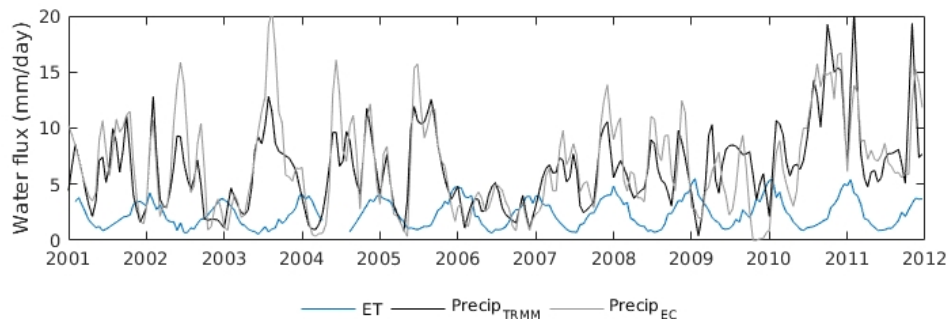
Fig. 1. Water fluxes at Tumbarumba (AU_Tum) sclerophyll forest: Evapotranspiration (ET, blue lines), satellite derived (Precip TRMM , black lines) and flux-tower (Precip EC , grey lines) precipitation (mm/day).
