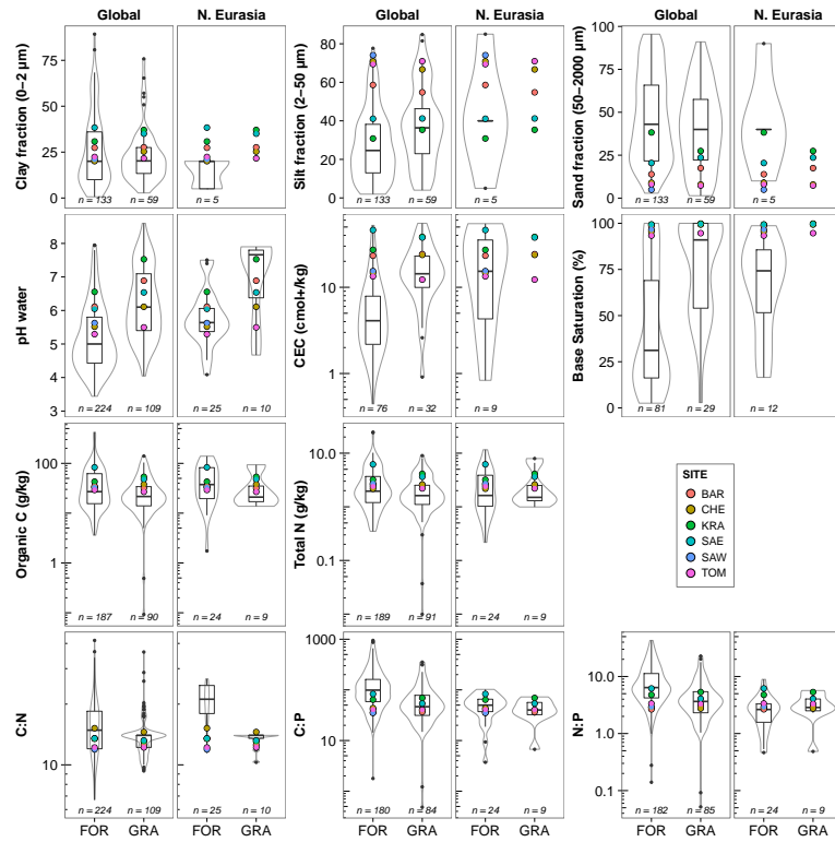
Fig. 1. Comparison of selected soil properties in topsoils (about 0 to –20 cm) of south-western Siberia (colored dots) and different vegetation types (FOR:forests; GRA: grasslands – box- and violin-plots) a
