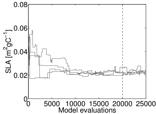
Figure 1. Sampled values of the specific leaf area (SLA) by DREAM_{(ZS)} parametrised with 4 chains, for the Oensingen site and the fixed homoscedastic error model (inversion HO1). The vertical dashed line indicates when convergence has been reached according to the \hat{R} statistic.
