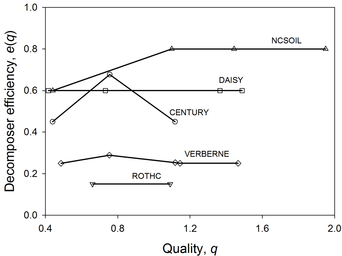
Fig. 1. Calculated carbon use efficiency e(q) = \text{CUE} as a function of quality q for the five models
