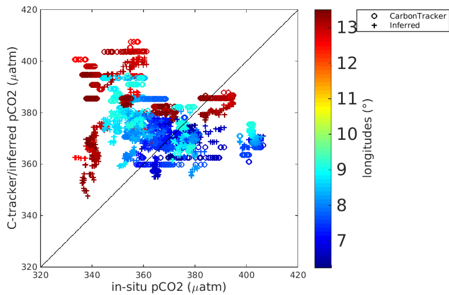
Fig. 2. Fig 2. The same as Fig. 1 but coloured as a function of longitude.
