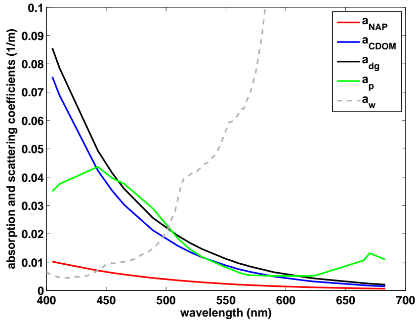
Fig. 4. Median IOP spectra from NOMAD dataset and absorption spectrum of pure water, a_w (Pope and Fry 1997). The absorption spectrum of particles (including phytoplankton) is indicated by a_p .
