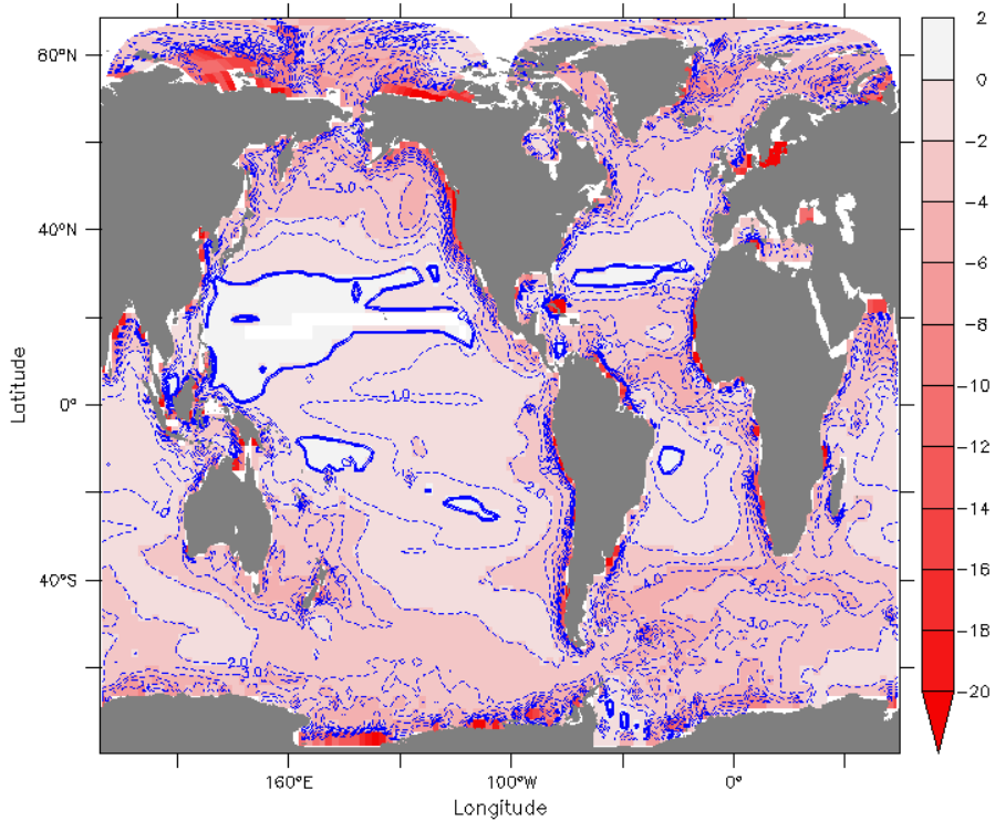
Fig. 5. Difference attenuation depth [m]; chl&CDM minus model run using Manizza 2005 parameterization (eq. 3 from manuscript).
