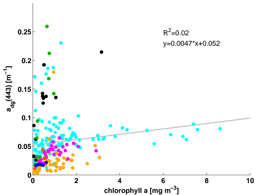
Fig. 1. Scatterplot of in-situ chlorophyll-a and a_{dg}(443) measurements from 244 stations where chlorophyll-a, a_{dg}(443) and k_d were measured concurrently. Data from NOMAD.
