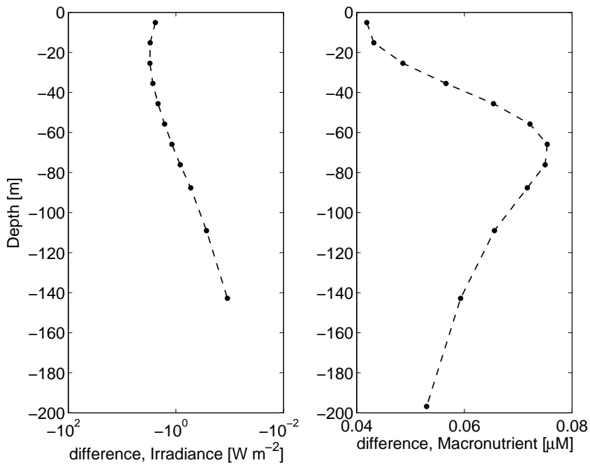
Fig. 7. Profiles of the change in globally averaged irradiance and macronutrient concentration, chl&CDM minus chl-only.
