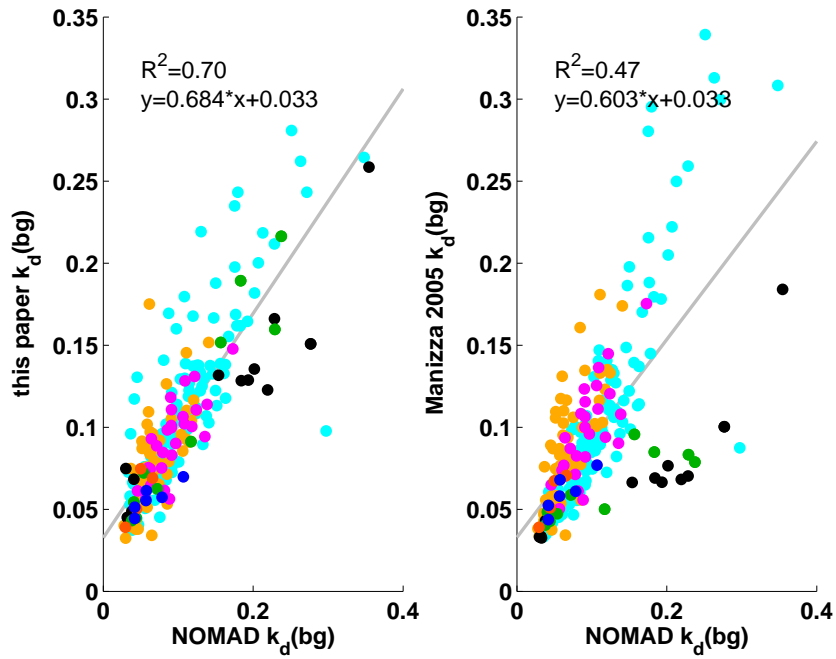
Fig. 2. Scatterplots comparing observed k_d(\text{bg}) from the NOMAD dataset and modeled k_d(\text{bg}) using two different parameterizations.
