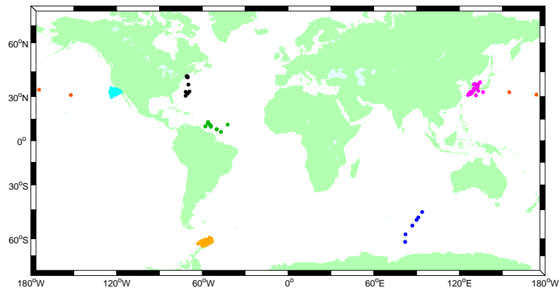
Fig. 3. Map of the 244 stations where measurements used to develop the k_d(\text{bg}) parameterization with CDM, equation 5, were made. Stations are spatially grouped and assigned an arbitrary color.
