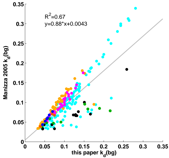
Fig. 6. Comparison of equation 3 and equation 5 applied to NOMAD in situ chlorophyll concentration and \text{adg}(443) measurements to calculate k_d(\text{bg}) .
