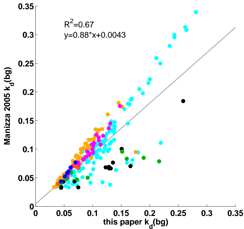
Fig. 6. Comparison of equation 3 and equation 5 applied to NOMAD in situ chlorophyll concentration and \text{adg}(443) measurements to calculate k_d (bg).
