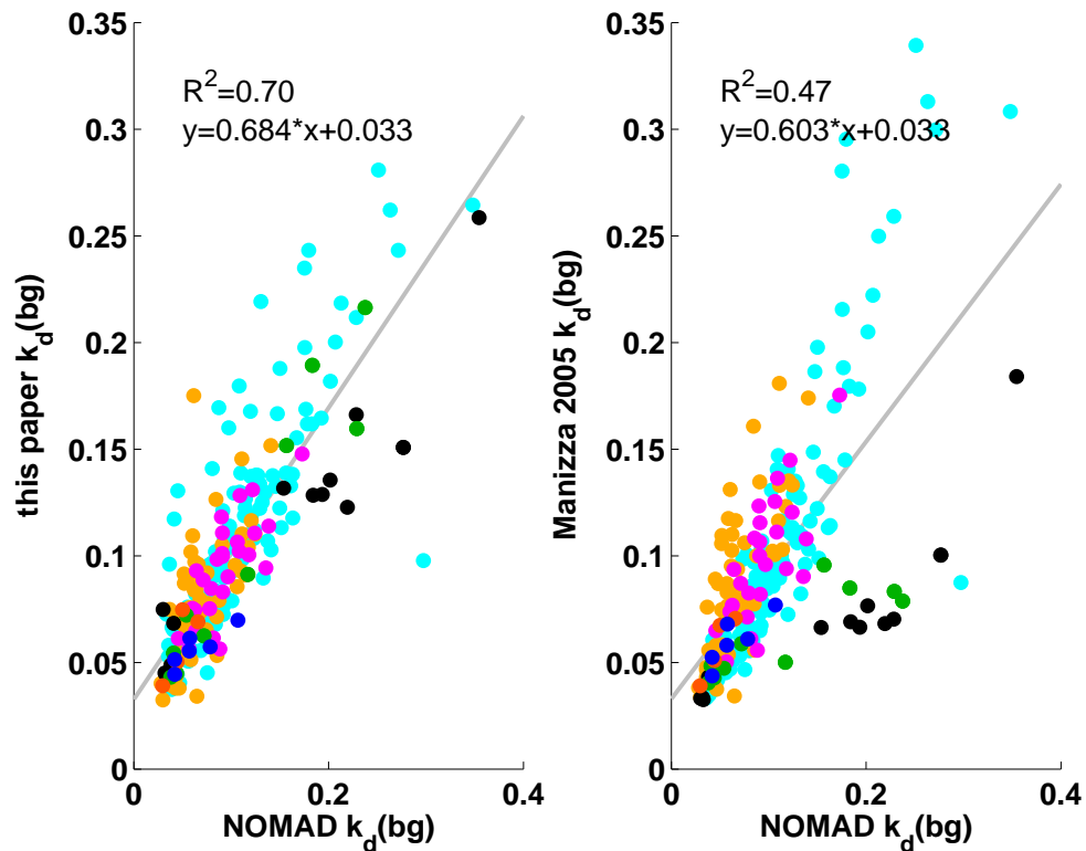
Fig. 2. Scatterplots comparing observed k_d (bg) from the NOMAD dataset and modeled k_d (bg) using two different parameterizations.
