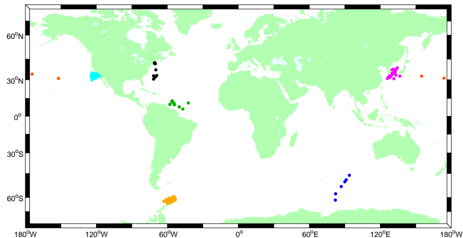
Fig. 3. Map of the 244 stations where measurements used to develop the k_d(bg) parameterization with CDM, equation 5, were made. Stations are spatially grouped and assigned an arbitrary color.
