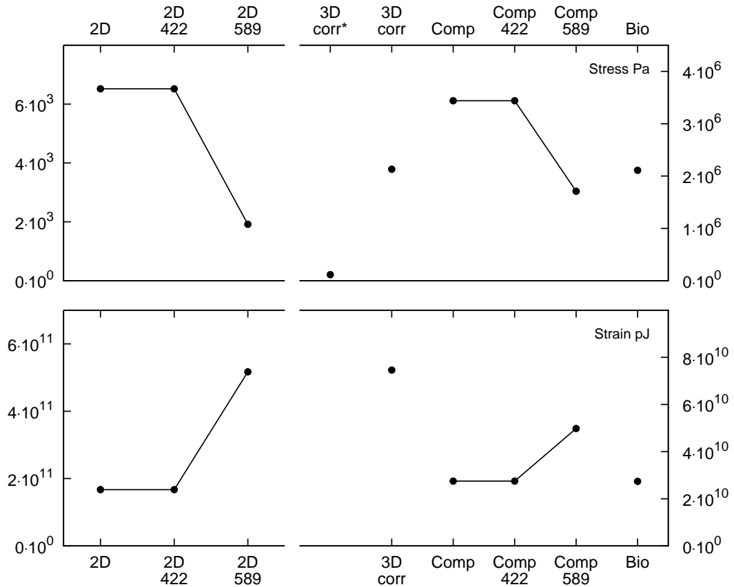
FIGURE 3. Stress and strain in models.
