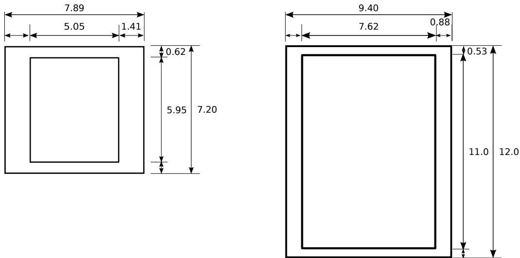
FIGURE 2. Estimated cell unit parameters.
