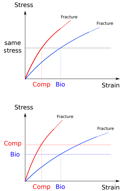
FIGURE 4. Stress-strain graphs.
