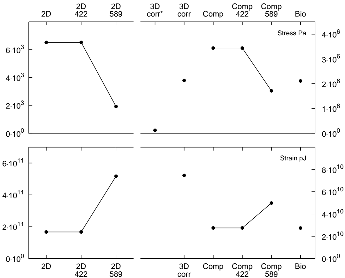
Fig. 3. Stress and strain in models.
