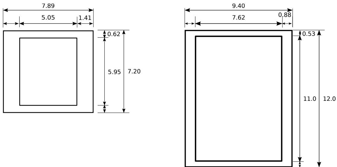
Fig. 2. Estimated cell unit parameters.
