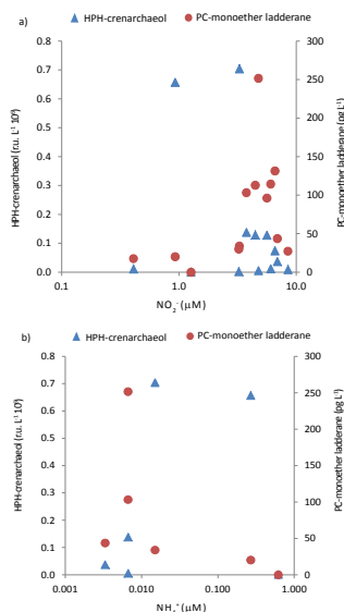
Fig. 1. Abundance of HPH-crenarchaeol (u.u. L -1 ) and PC-monoether ladderane (pg L -1 ) lipids versus (a) \text{NO}_2^- ( \mu\text{M} ) and of (b) \text{NH}_4^+ ( \mu\text{M} ) at the coastal site.
