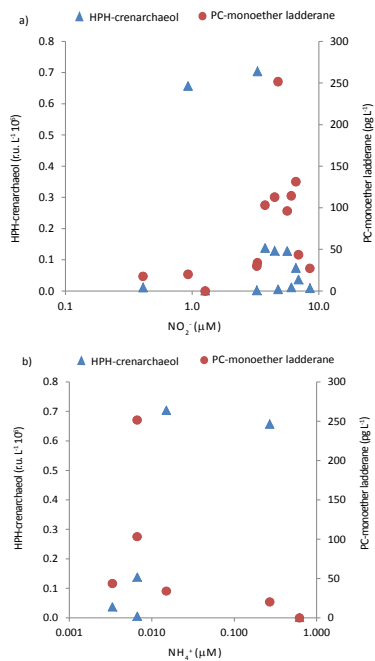
Fig. 1. Abundance of HPH-crenarchaeol (r.u. L -1 ) and PC-monoether ladderane (pg L -1 ) lipids versus (a) \text{NO}_2^- ( \mu\text{M} ) and of (b) \text{NH}_4^+ ( \mu\text{M} ) at the coastal site.
