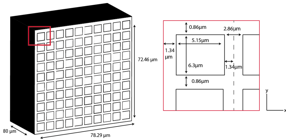
Fig. 2. Dimensions used in the 3D corridor model. Units = \mu m
