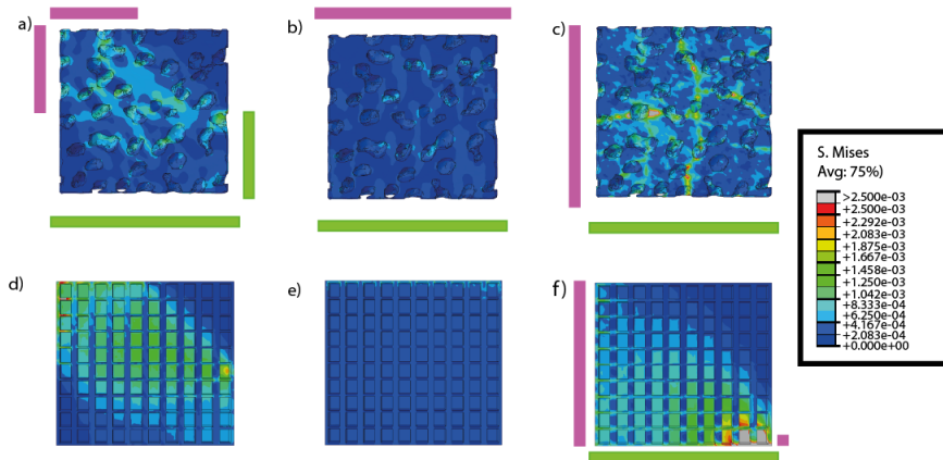
Fig. 1. The von Mises Stress patterns on the biologically realistic model (a, b & c) and the compartmentalised model (d, e & f) in different loading situations. Units = N \mu m^{-2} .
