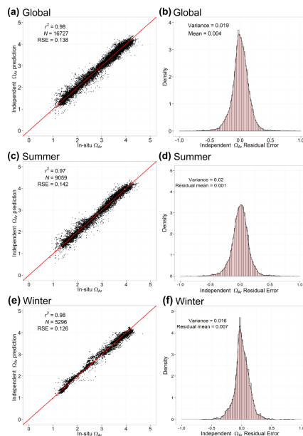
Figure 3: Statistical plots comparing global \Omega_{A_e} values calculated via the in-situ network of C_T and A_T measurements, and independently predicted C_T and A_T values via the approach of Sasse et al (2013b). (a) Global independent predictions versus in-situ values, where the red line represents y = x relationship (b) Global distribution of the independent residual errors (c,e) Winter and Summer independent predictions versus in-situ values (d,f) Winter and Summer distribution of the independent residual errors. Summer and winter months were defined as June through to August and December through to February for Northern Hemisphere respectively, while Southern Hemisphere differed by 6 months.
