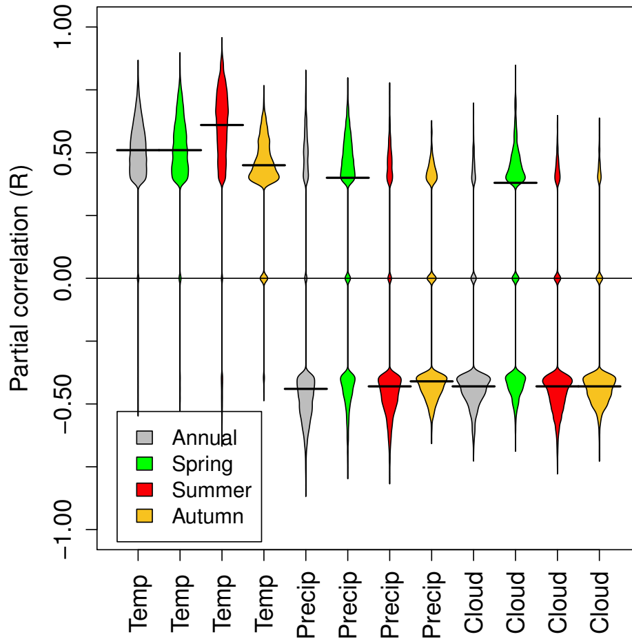
Figure 7: Bean plots of the multi-modal distribution for significant (95% significance) partial correlation between annual de-trended GPP (GPPsat) and the values of each de-trended environmental variable after eliminating the influence of the other variables. A bean plot is an alternative to the box plot and is fundamentally a one dimensional scatter plot. Here it is preferred over a box plot as it helps to visualize a multi-modal distribution. The thickness of a 'bean' is a function of the frequency of the specific value, that is the thicker a 'bean' is for a value, the relatively higher is the number of grid-points having that value. The values shown are the Pearson's correlation coefficients which are based on the linear least squares trend fit. Correlation values range from -1 to +1 . Values closer to -1 or +1 indicates strong correlation while those closer to 0 indicates weak correlation. The color of the box indicates the season of the environmental variable being investigated (Annual = grey; Spring = green, Summer = red; Autumn = amber). The short horizontal black lines for each 'bean' is the median of that distribution.
