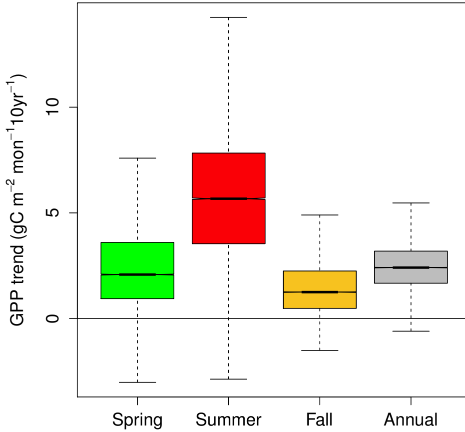
Figure 5: Box plot showing grid distributions of seasonal GPP trends for GPPsat. The GPP trends are expressed in \text{g C m}^{-2} \text{ month}^{-1} 10 \text{ yr}^{-1} . The black band and middle notch represent the 2nd quartile or median, box extents mark the 25th (1st quartile) and 75th (3rd quartile) percentiles. Whiskers extend from the smallest non-outlier value to the largest non-outlier value. The colors, green, red, orange and gray represent spring, summer, autumn and annual seasonal trends respectively. As described in Sect. 2.1.2, GPP trends for winter have not been assessed in this study.
