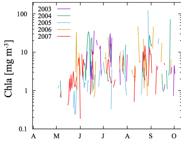
Figure R4. Time series (2003–2007) of chla for the point of Bering Strait (168°N, 170.2°W).
