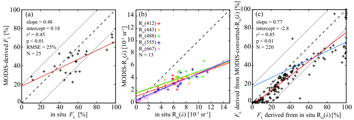
Figure R2. Scatter plots of (a) satellite-derived F_L vs. in situ observed surface F_L ( r^2 = 0.45 , p < 0.01 , N = 25 , RMSE = 25\% ), (b) satellite-derived R_{rs}(\lambda) vs. in situ measured R_{rs}(\lambda) ( N = 13 , slopes and intercepts for each \lambda are listed in Table R1), and (c) F_L derived from MODIS-converted- R_{rs}(\lambda) vs. F_L derived from in situ R_{rs}(\lambda) ( r^2 = 0.85 , p < 0.01 , N = 220 ). Dashed lines are 1:1 lines, dotted lines indicate \pm 20\% from 1:1 (Fig. R2a and c), and coloured solid lines represent regression line, respectively. The regression line of Fig. R2a is also shown in Fig. R2c with the blue solid line for comparison.
