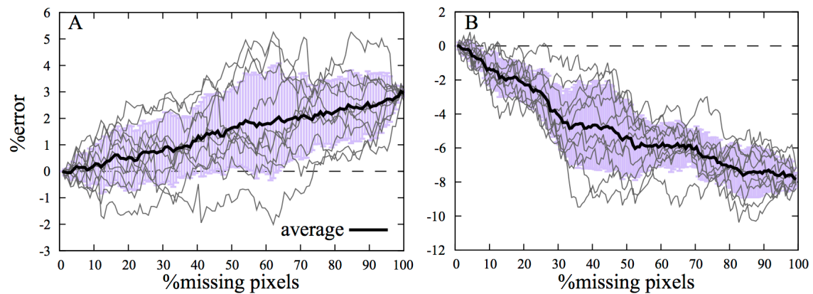
Figure R1. Relationships between the percentage of replaced pixels from original PP_{eu} to annual median PP_{eu} and percent error from “true” APP. Grey lines indicate the each simulation and thick black lines represent the average of the error. Error bars coloured in violet represent standard deviations.
