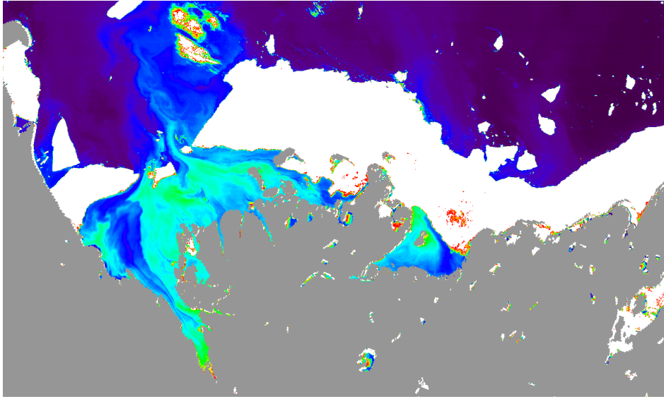
Fig. 1. Radiance recorded at the top of the atmosphere (MODIS-Aqua, band 2: 859 nm, 24 June 2004) at a spatial resolution of 250 m: zoom on the Mackenzie River mouth (delta zone and stamukha).
