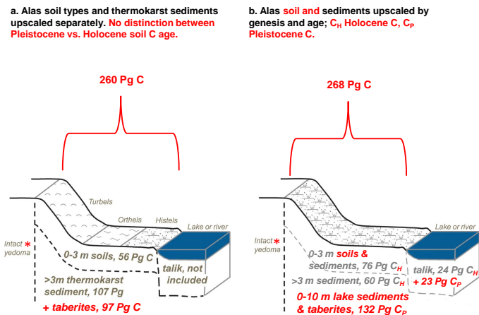
Figure 2. Modified from Hugelius et al. (Biogeosciences Discuss. Fig. 2): "Conceptual diagram illustrating how organic soil/sediment C in Yedoma region alases is described and estimated by (a) Hugelius et al. (2014) and (b) by Walter Anthony et al. (2014)." Our suggested corrections to the figure are shown in red font. It is interesting to note that the total values for alas carbon pool size are similar in a and b despite being based on independent soil carbon data sets. Walter Anthony et al. (2014) never suggested that the 159 Pg Holocene C described for yedoma region alases should be added to existing estimate of regional carbon stocks. In fact, we showed clearly that our new work did not change previous estimates of the total regional carbon pool size estimate; rather, it shed light on the ages and origins of the carbon subpools therein. The novelty of Walter Anthony et al. (2014) was distinguishing Holocene vs. Pleistocene carbon age and its implication for greenhouse gas fluxes during the past 10,000 years.
