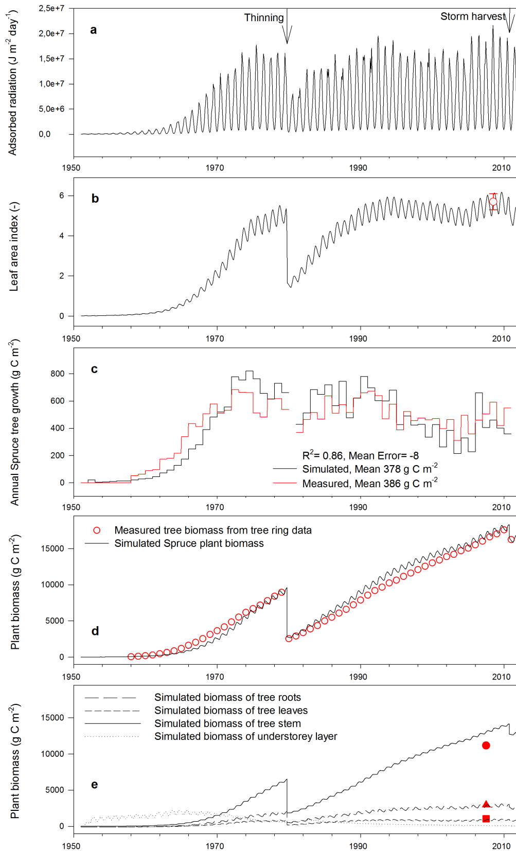
Figure 2. a) Simulated (black line) Spruce adsorbed radiation; b) simulated and measured (red hollow circle) leaf area index; c) annual Spruce tree growth rate; d) total plant biomass; e) plant biomass for different components. In Fig. 2e, the solid red symbols show the calculated
