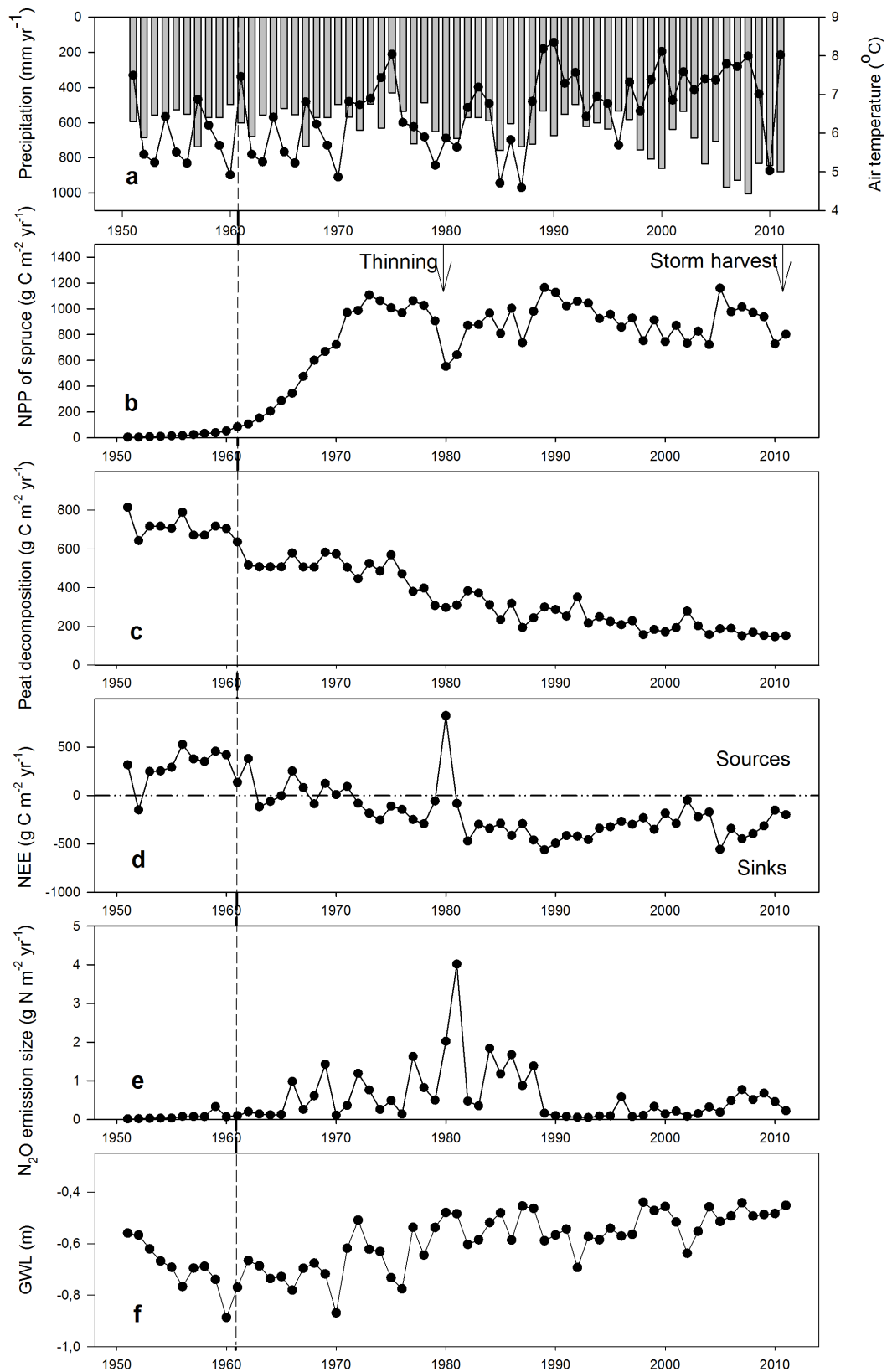
Figure 5. For the period 1951 to 2011: a) Annual precipitation and air temperature; b) the simulated annual NPP of Spruce trees; c) annual peat decomposition rate; d) annual NEE; e) annual N 2 O emissions; f) annual GWL. The dashed reference line separates the duplicated
