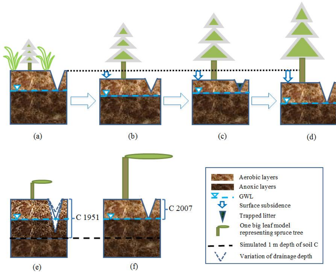
Figure 1. Conceptual representation of the dynamics of plants and peat soil development over a forest rotation period. The upper figures (1a, 1b, 1c, 1d) represent the conceived reality and 1e and 1f represent the CoupModel conceptualization. For all the figures, Spruce tree and understorey vegetation, e.g. grasses are considered but for clarity, understorey vegetation is only shown in Fig. 1a. ‘C 2007’ in Figure 1f represents the measured total soil C in the upper 0.5 m of the soil profile in 2007, and ‘C 1951’ is the total soil C in the upper 1 m of the soil profile, as back-calculated from the equation: \text{‘C 2007’} + (2007-1951) \times \text{IPCC EF's} . Any variation of climate during the forest development in this conceptual figure is not considered.
