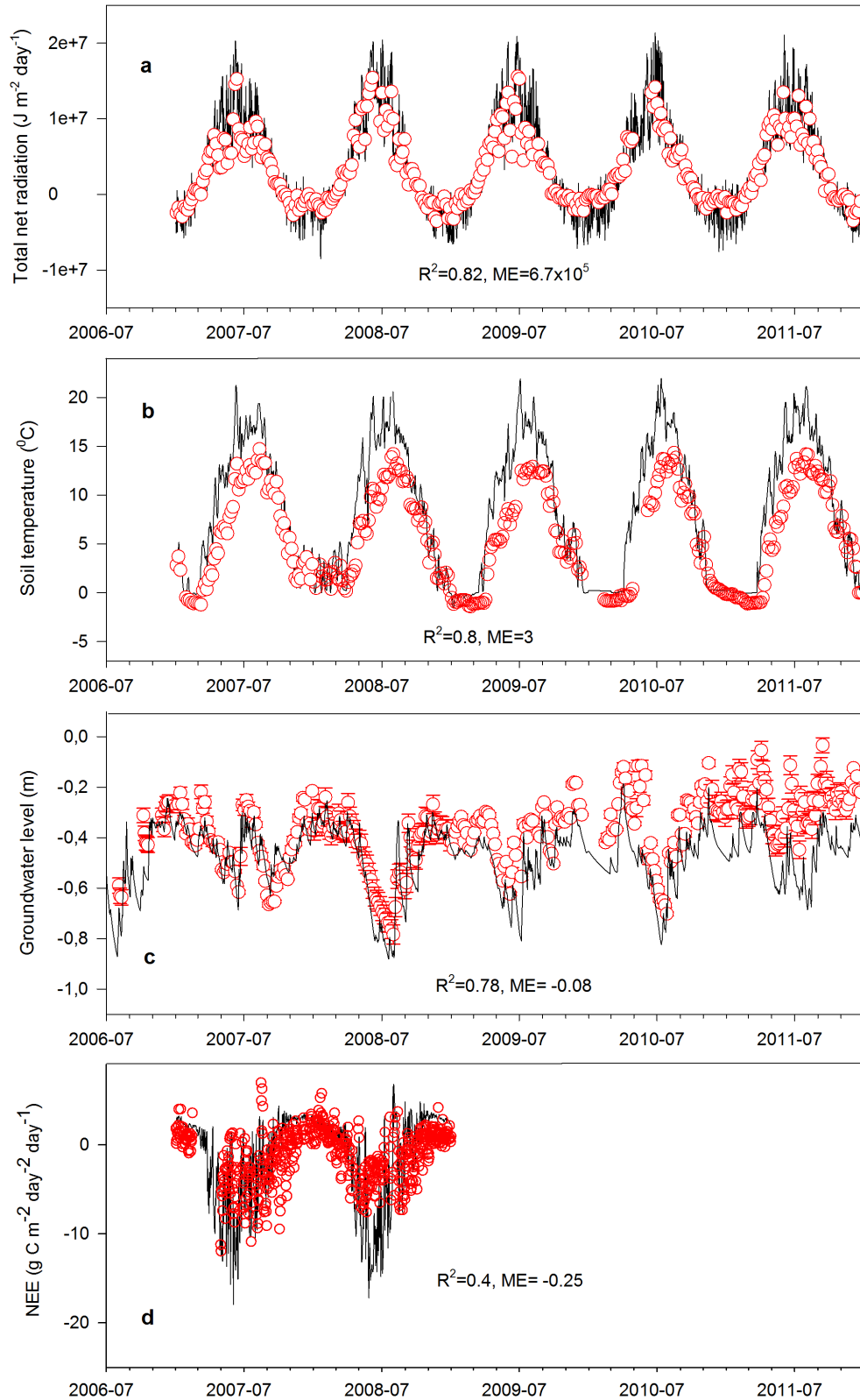
Figure 4. a) Simulated (black line) and measured (red hollow circle) total net radiation; b) soil surface temperature (0-5 cm depth; c) GWL ; d) NEE. Measured data used to create these plots are 5-day averages, except for NEE where daily averages have been used.
