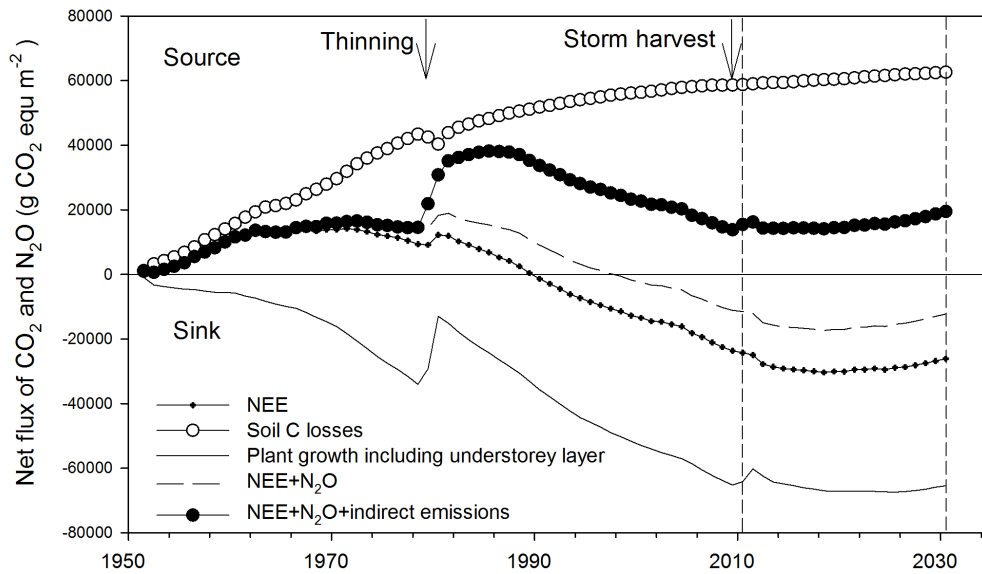
Figure 6. Simulated total GHG balance for the forest ecosystem from 1951 to 2011 and extended to 2031. The simulated results of 2011 to 2031 are obtained by running the reference model with extended meteorological files using meteorological data from 1991 to 2011 duplicated to represent the climate of 2011 to 2031. It should be noted that the GHG balance presented in this figure assumes no final harvest.
