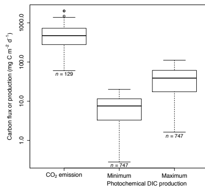
Figure 5. Box-and-whiskers plots of total measured CO 2 emissions, and minimum and maximum simulated photochemical DIC production, showing the median and 1 st and 3 rd quartiles with the whiskers set at \pm 1.5 times the interquartile range and data outside this range given as circles. Note the log scale on the y-axis.
